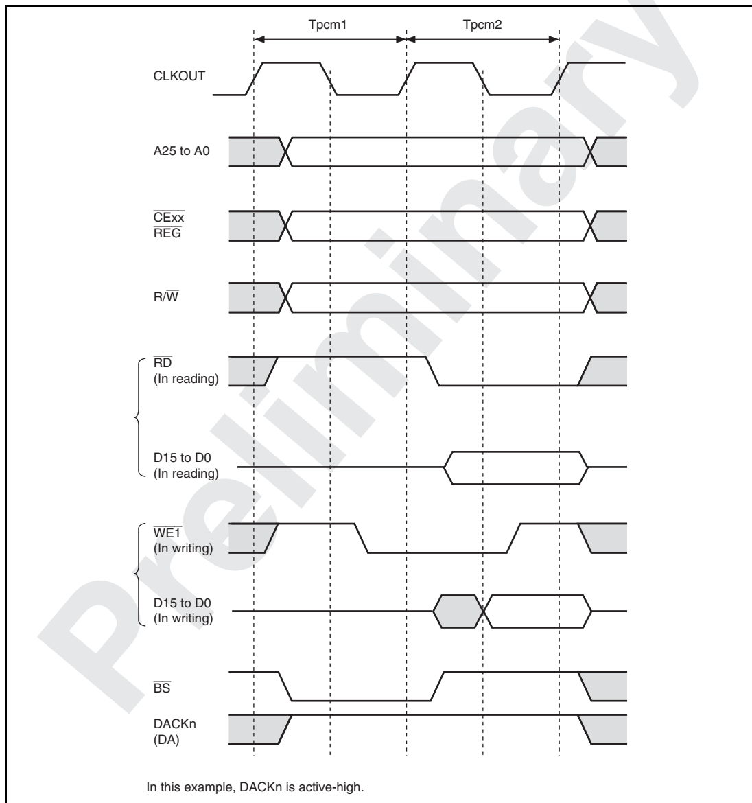
Figure 11.17 Basic Timing for PCMCIA Memory Card Interface
