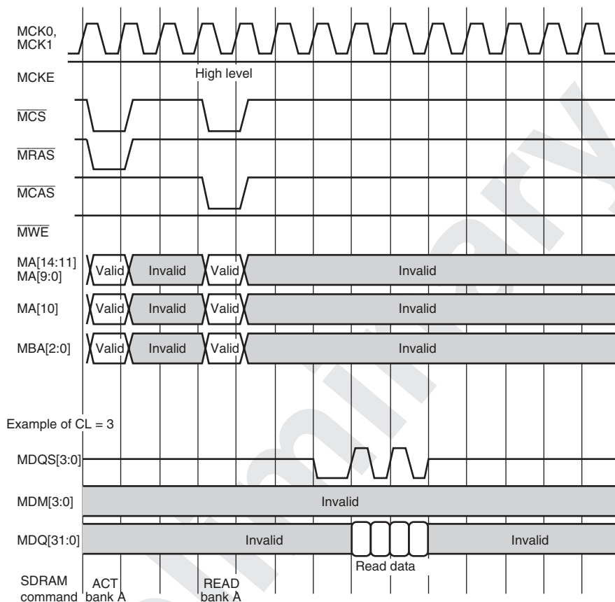
Figure 12.8 Waveforms for 1/2/4/8/16-Byte Reading (When the Bus Width is Set to 32 bits)
