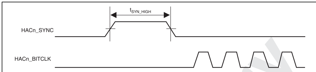
Figure 32.60 HAC Warm Reset Timing
