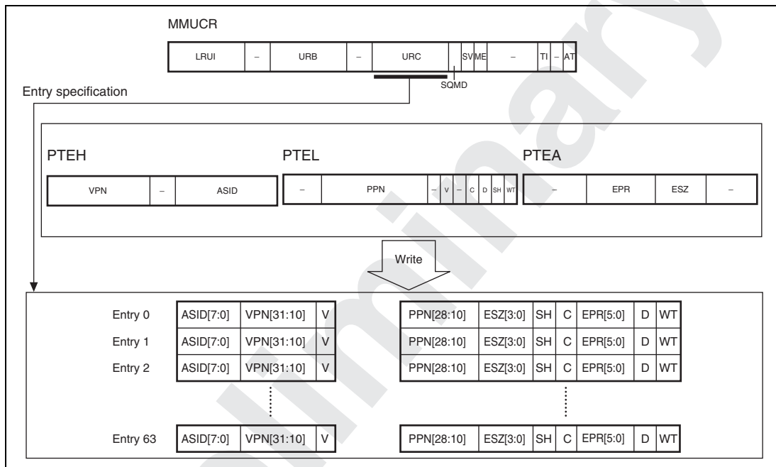
Figure D.8 Operation of LDTLB Instruction (TLB Extended Mode)
