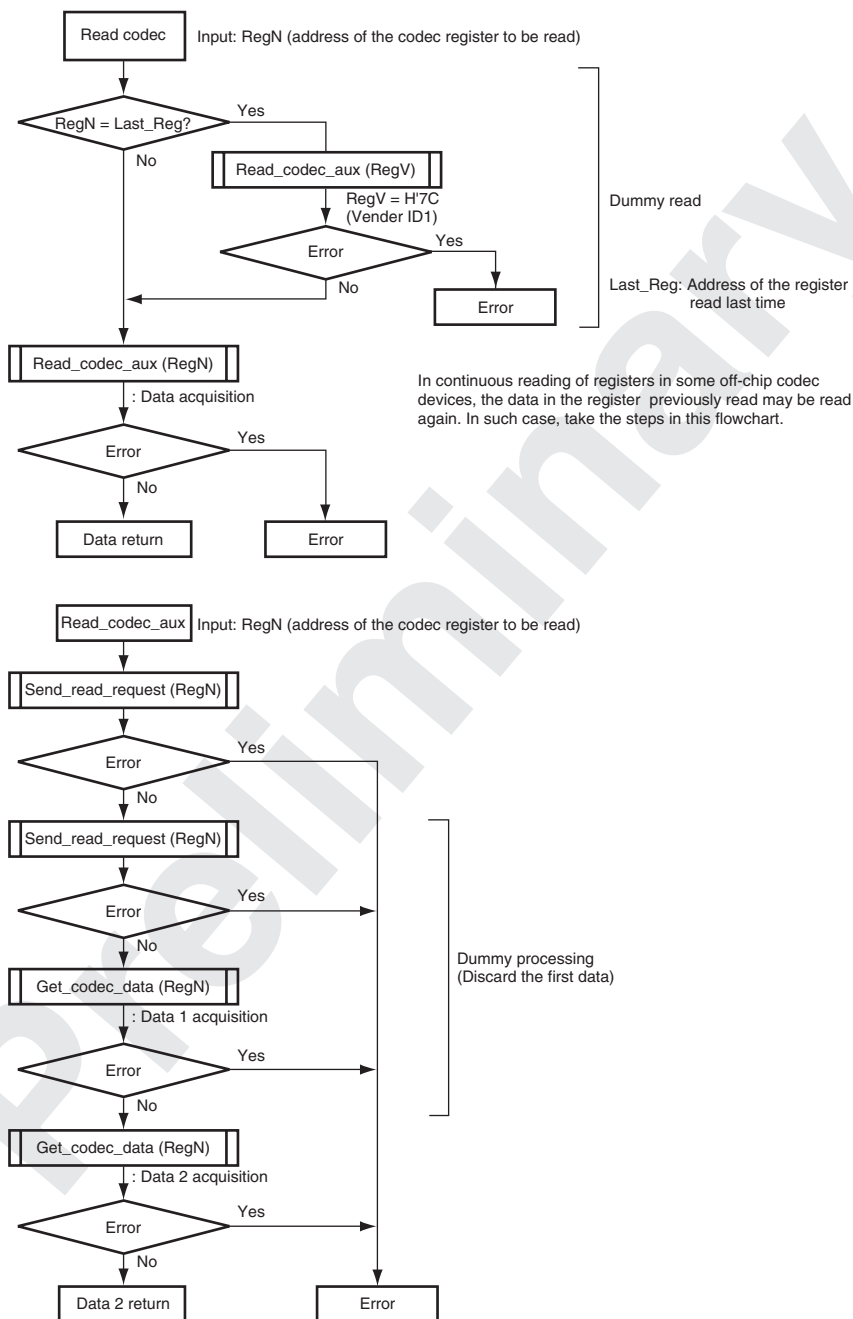
Figure 25.5 Sample Flowchart for Off-Chip Codec Register Read (1)
