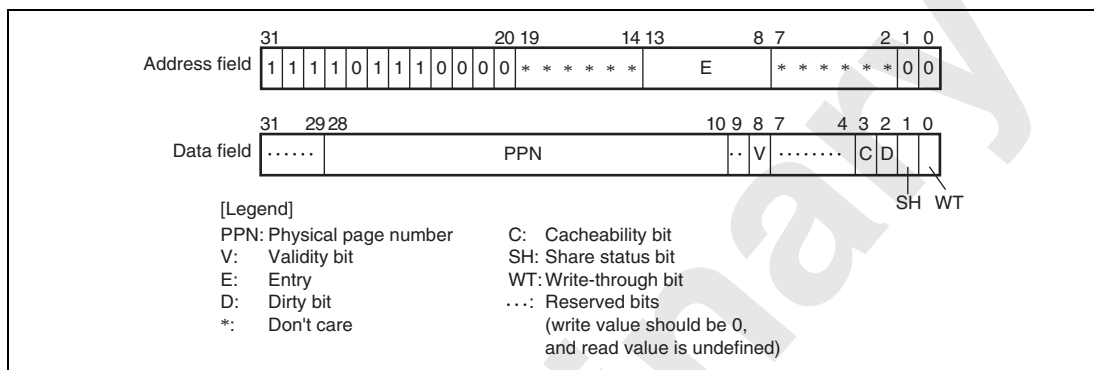
Figure D.11 Memory-Mapped UTLB Data Array 1 (TLB Extended Mode)
