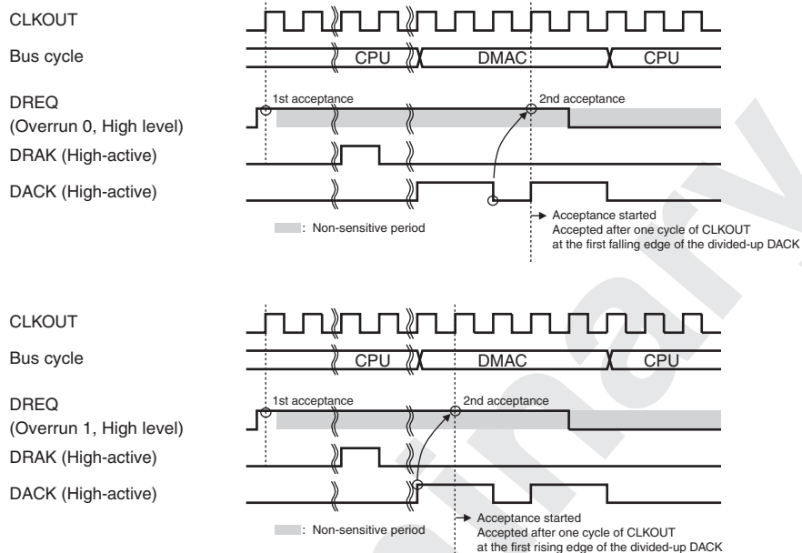
Figure 14.17 Example 2 of DREQ Input Detection in Cycle Steal Mode Level Detection (Word Transfer in 8-Bit Bus Width, Longword Transfer in 8/16-Bit Bus Width, 16/32-Byte Transfer in 8/16/32/64-Bit Bus Width: DACK of DMA1 Transfer Divided)
