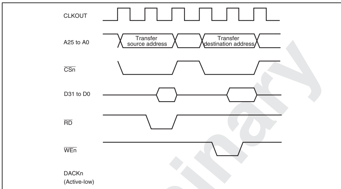
Figure 14.5 Example of DMA Transfer Timing in Dual Address Mode (Source: Ordinary Memory, Destination: Ordinary Memory)
