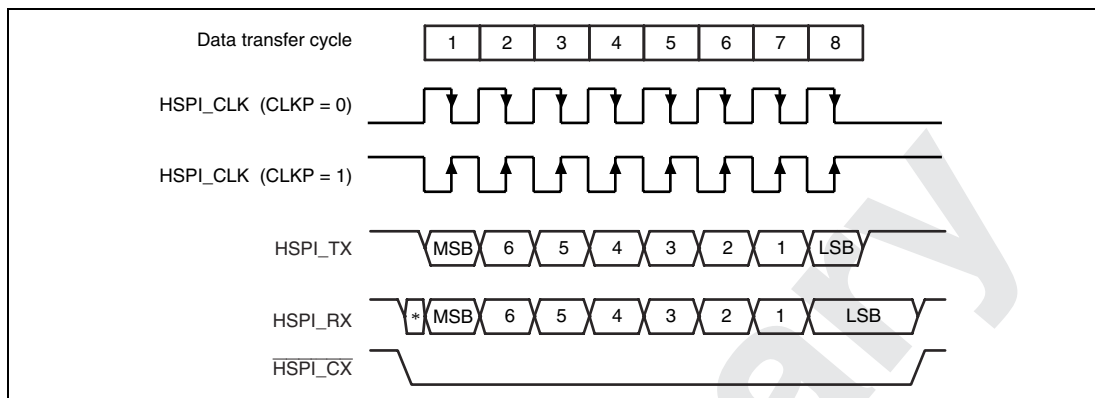
Figure 23.5 Timing Conditions when FBS = 1
