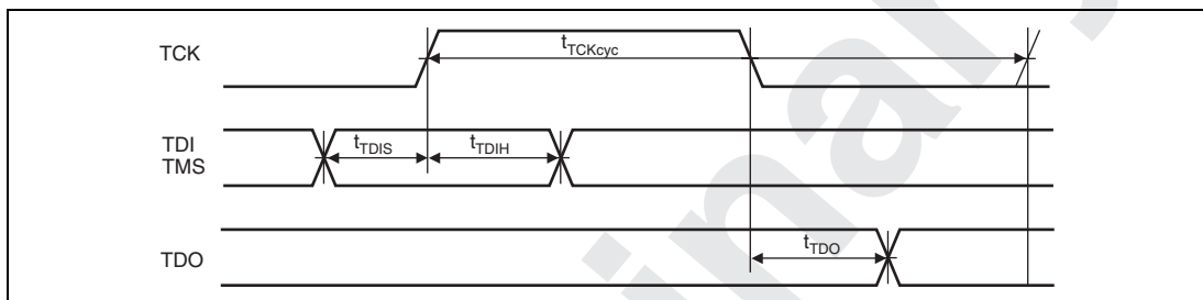
Figure 32.46 H-UDI Data Transfer Timing
