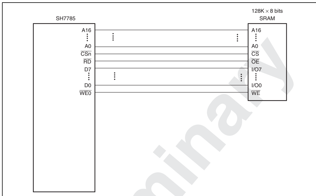
Figure 11.8 Example of 8-Bit Data Width SRAM Connection
