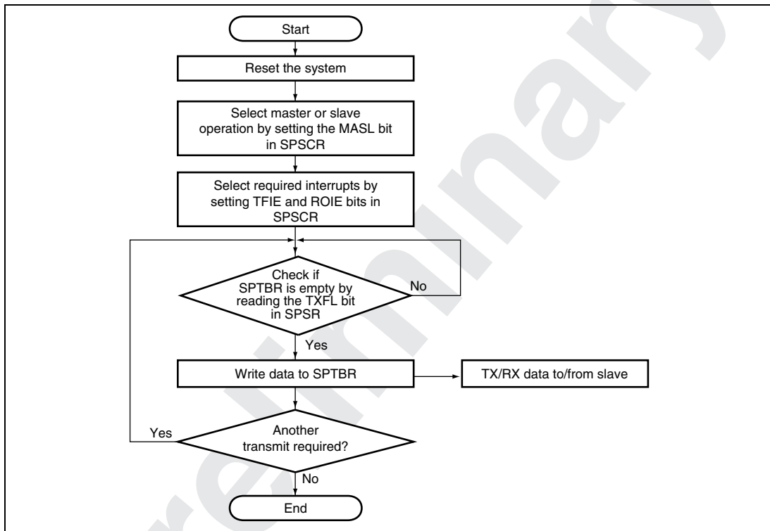
Figure 23.2 Operational Flowchart
