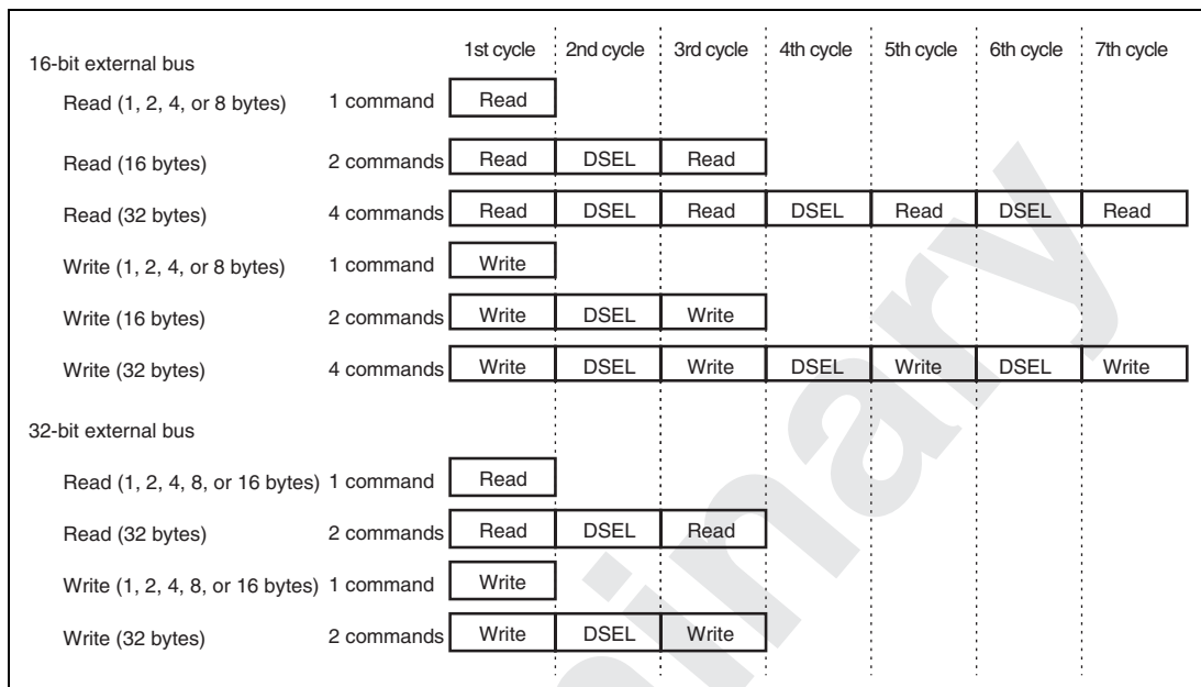
Figure 12.5 Read/Write Command Issued to the SDRAM in Response to the Request from the SHwy Bus
