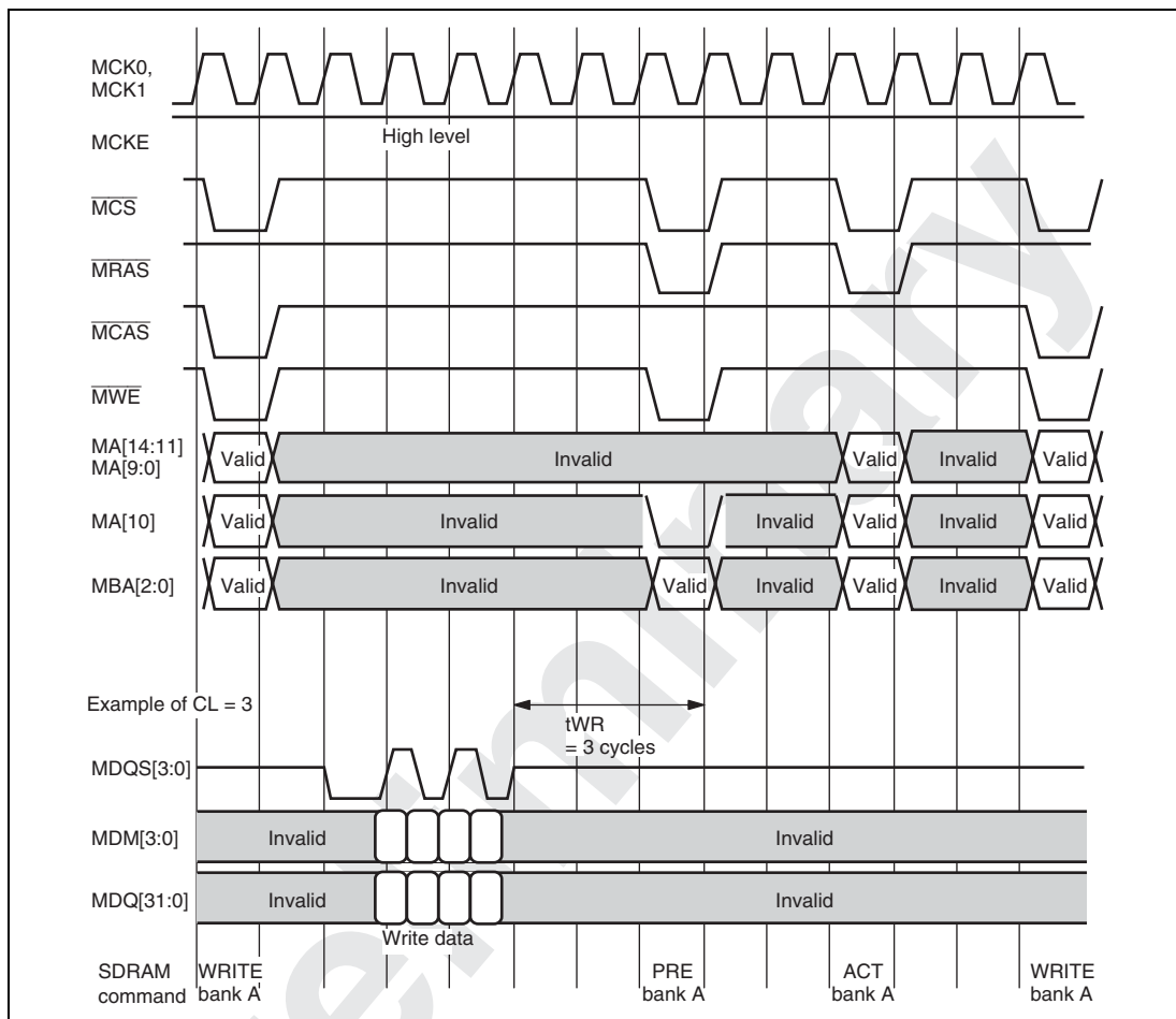
Figure 12.16 tWR
