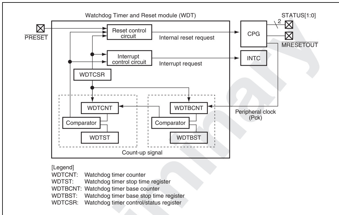
Figure 16.1 Block Diagram of WDT
