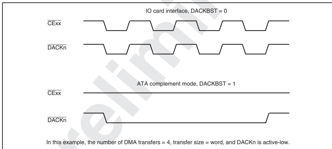
Figure 11.15 \overline{CE1x} and \overline{DACKn} Output during DMA Transfer in Access to Space where ATA Complement Mode is Set
