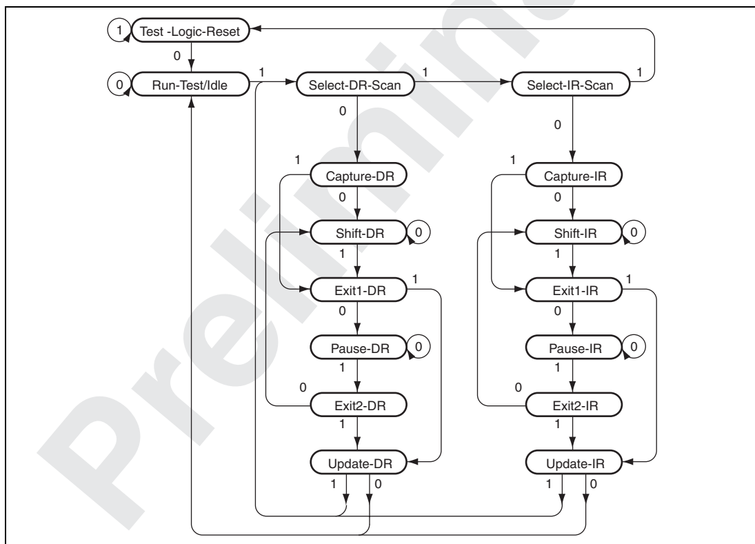
Figure 30.3 Diagram of Transitions of TAP Controller State
