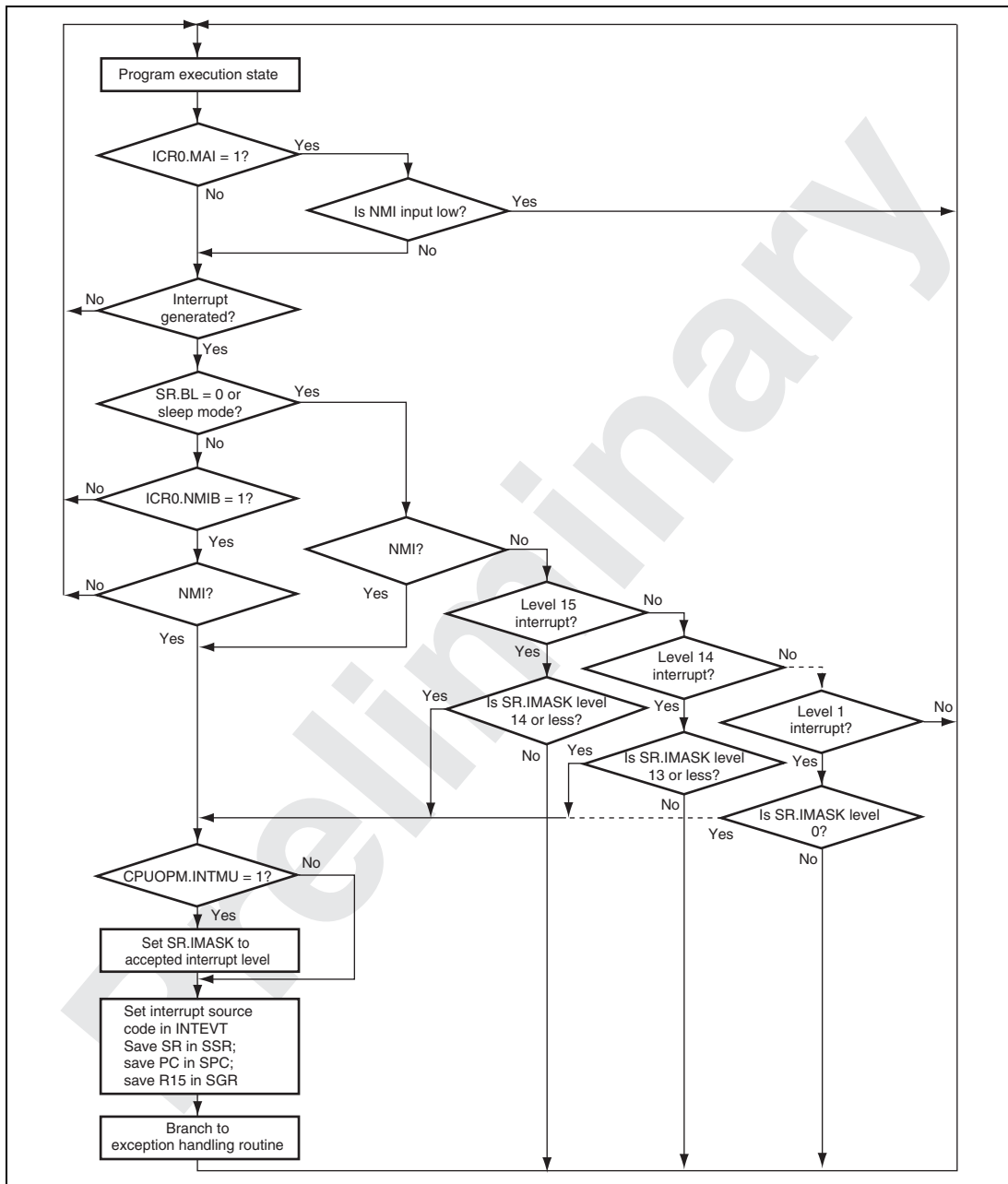
Figure 10.5 Flowchart of Interrupt Operation
