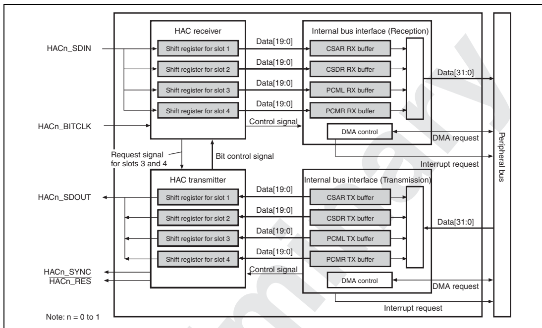
Figure 25.1 Block Diagram
