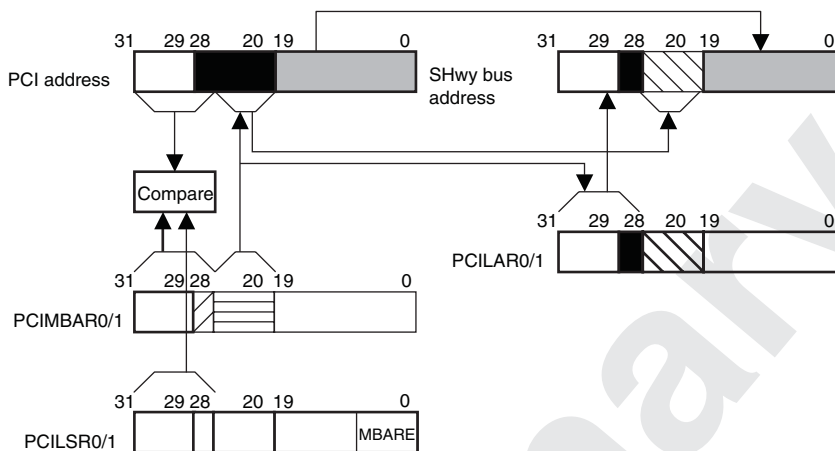
Figure 13.11 PCI Bus to SHwy Bus Address Translation
