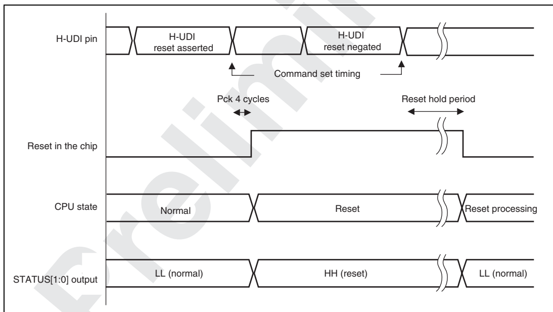
Figure 30.4 H-UDI Reset
