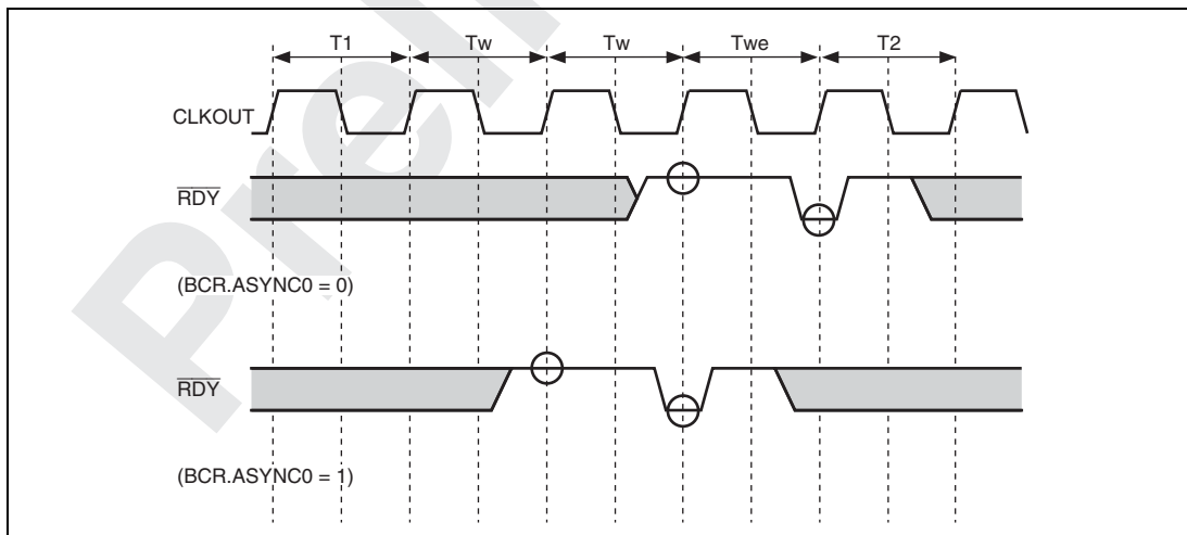
Figure 11.4 \overline{\text{RDY}} Sampling Timings with ASYNC n Settings (Two Wait Cycles Inserted by CS n WCR.)
