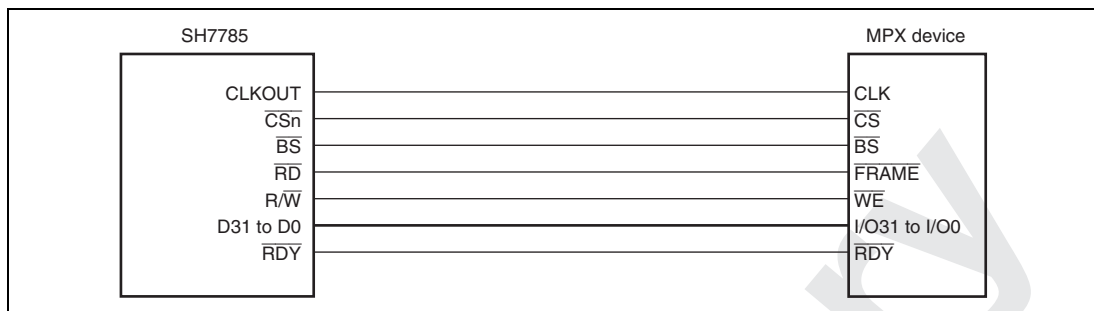
Figure 11.22 Example of 32-Bit Data Width MPX Connection
