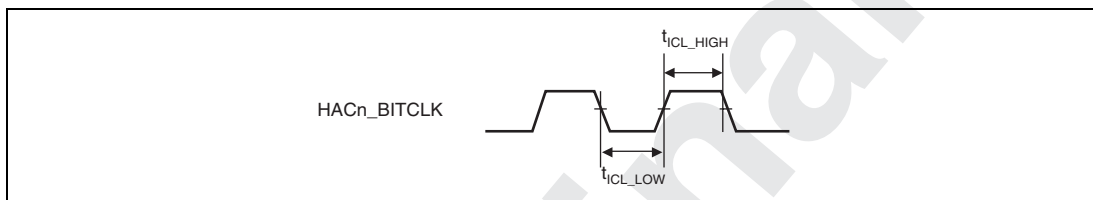
Figure 32.61 HAC Clock Input Timing
