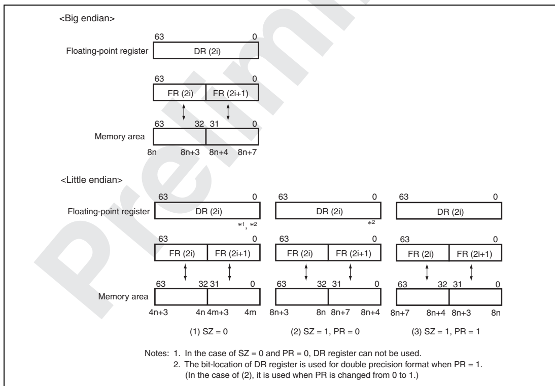
Figure 6.5 Relation between SZ Bit and Endian
