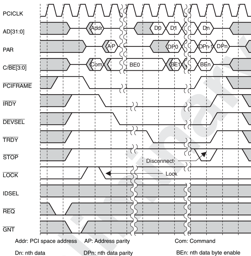
Figure 13.25 Target Memory Read Cycle in Host Mode (Burst)
