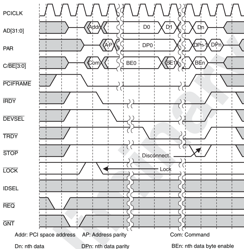
Figure 13.26 Target Memory Write Cycle in Host Mode (Burst)
