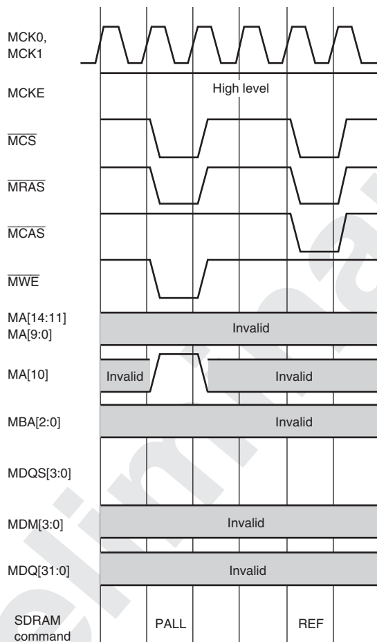
Figure 12.12 Auto-Refresh Operation
