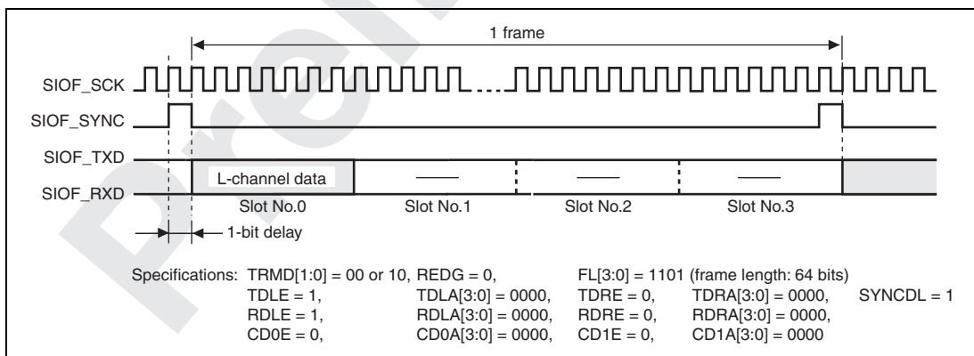
Figure 22.15 Transmit and Receive Timing (16-Bit Monaural Data)
