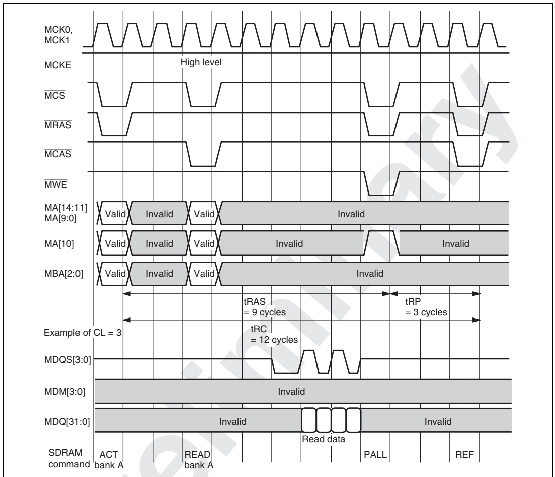
Figure 12.17 t_{RC}
