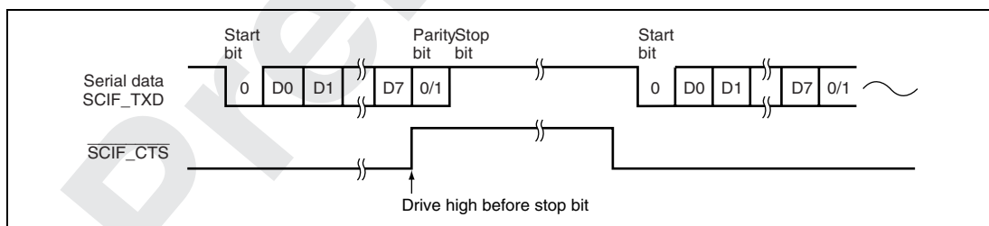
Figure 21.11 Example of Operation Using Modem Control ( SCIF_CTS ) (Only in Channel 0)
