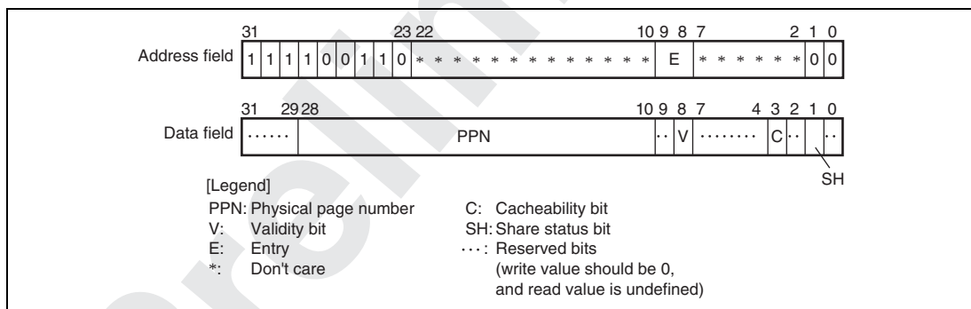
Figure D.9 Memory-Mapped ITLB Data Array 1 (TLB Extended Mode)
