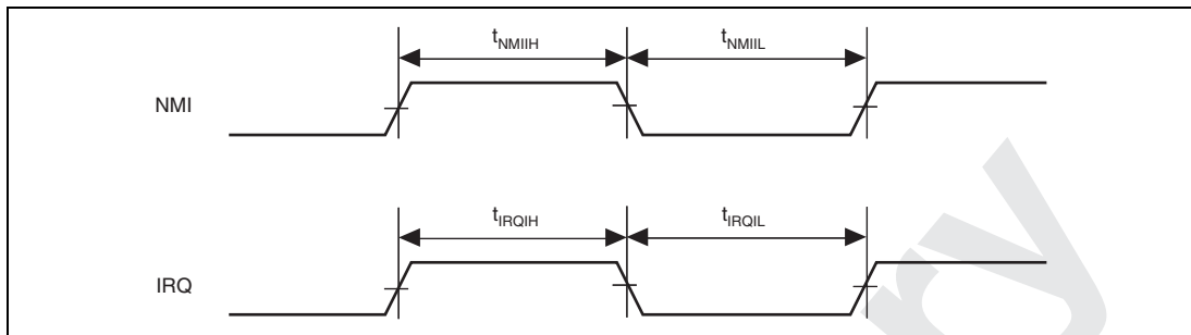
Figure 32.35 Interrupt Signal Input Timing (2)
