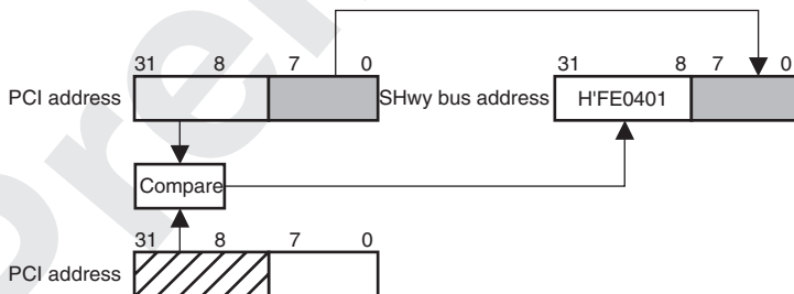
Figure 13.12 I/O Access from PCI Bus to SHwy Bus
