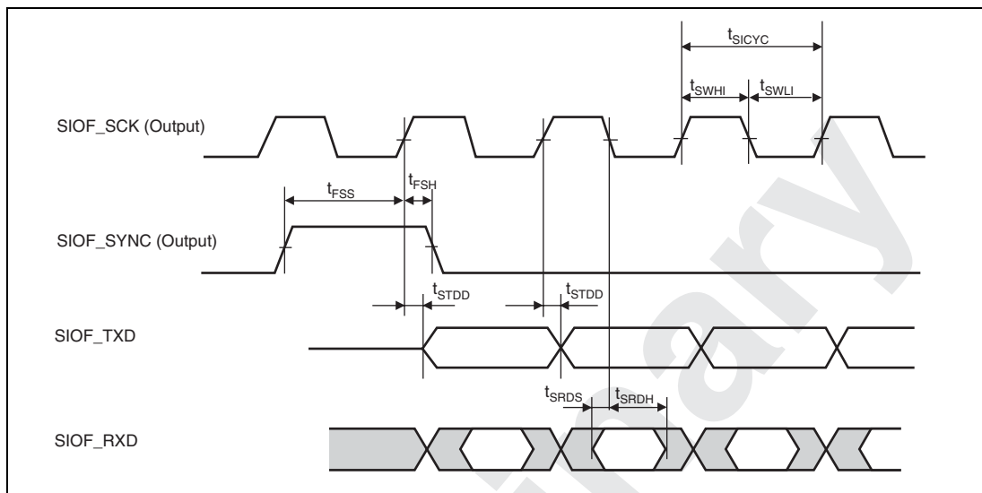
Figure 32.55 SIOF Transmission/Reception Timing (Slave Mode 1, Slave Mode 2)
