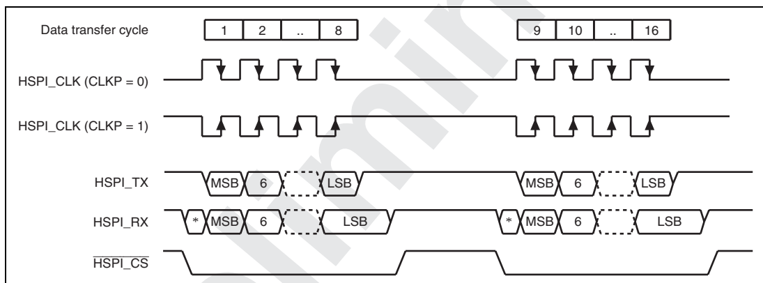
Figure 23.6 Timing Conditions when FBS = 1 (Continuous Transfer)
