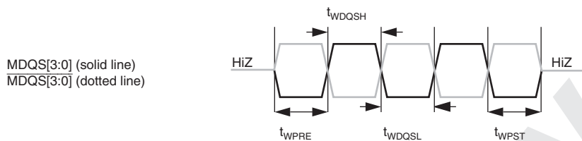
Figure 32.31 MDQS Output Waveform (Write)
