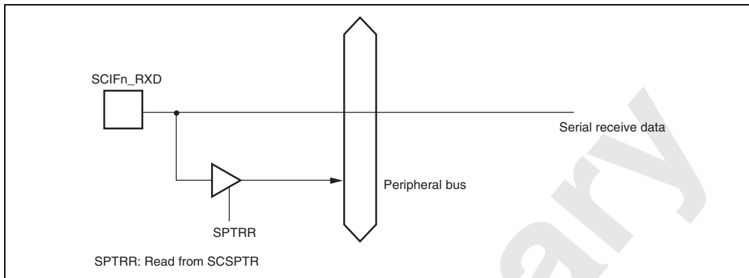
Figure 21.6 SCIFn_RXD Pin (n = 0 to 5)
