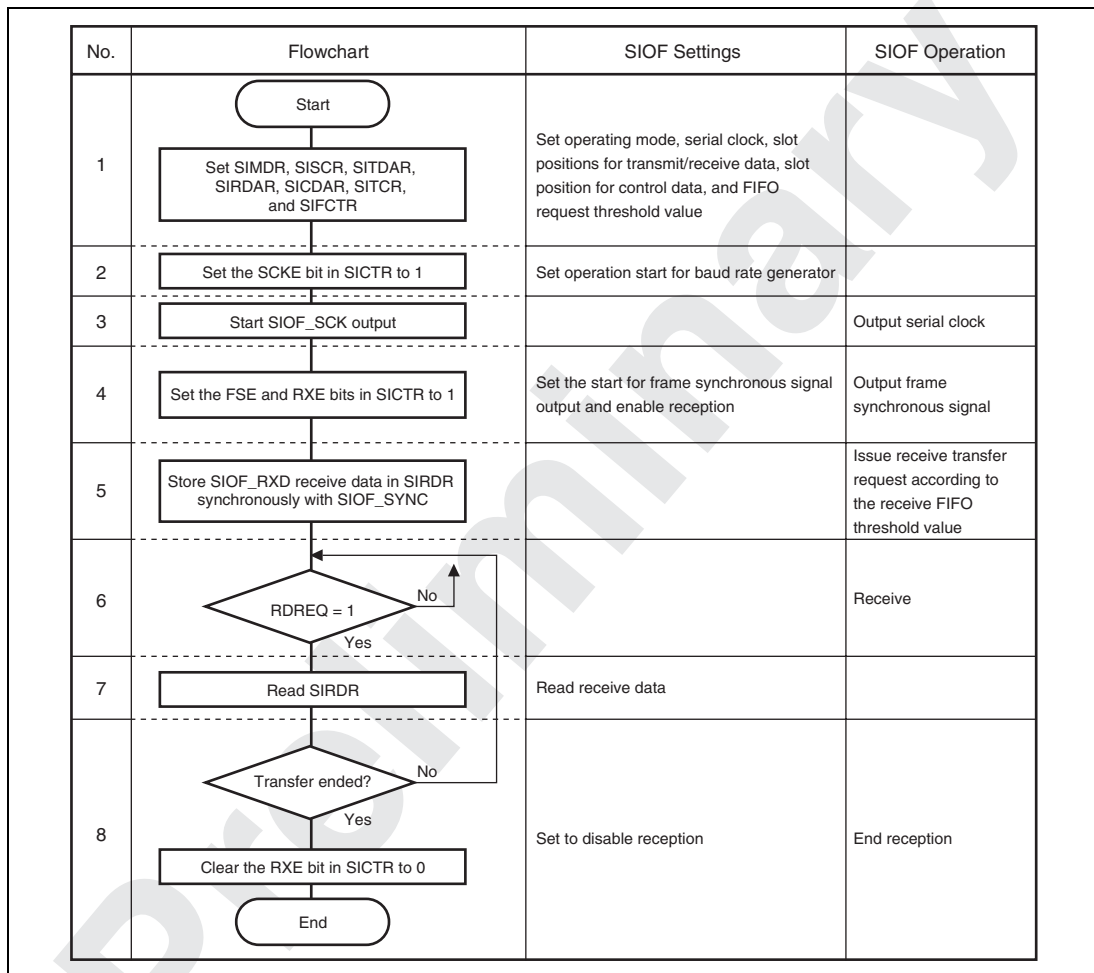
Figure 22.10 Example of Receive Operation in Master Mode
