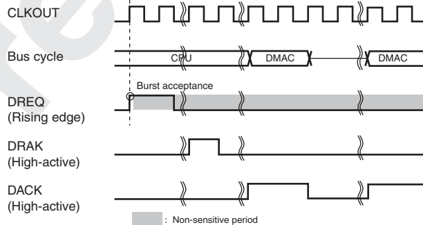
Figure 14.19 Example of DREQ Input Detection in Burst Mode Edge Detection
