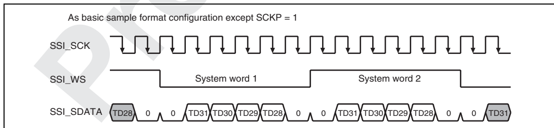
Figure 26.10 Inverted Clock
