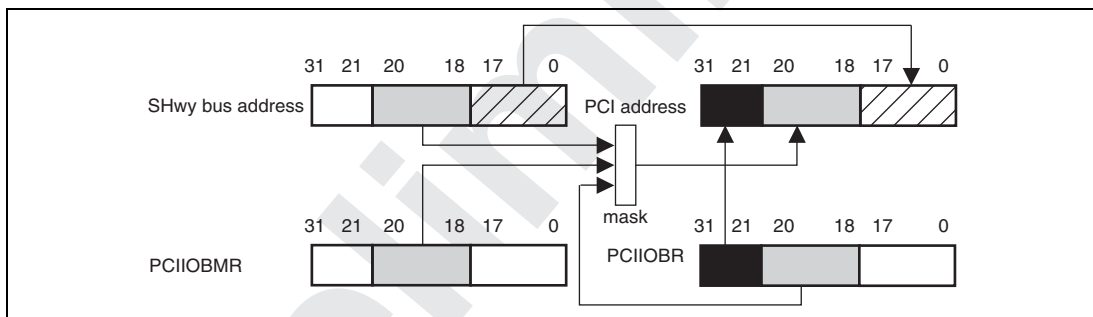
Figure 13.6 Access from SHwy Bus to PCI I/O Space (PCI Bus)
