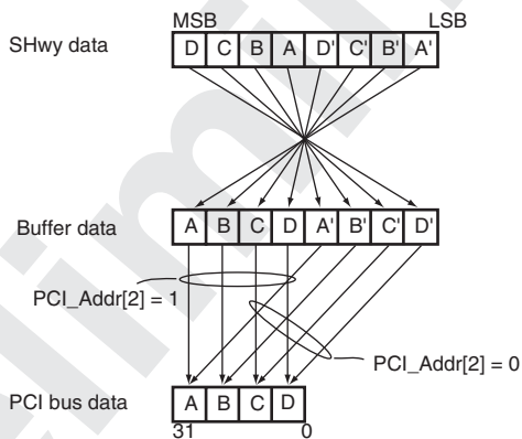
Figure 13.8 Endian Conversion from SHwy Bus to PCI Local Bus (Byte Swapping: TBS = 1)
