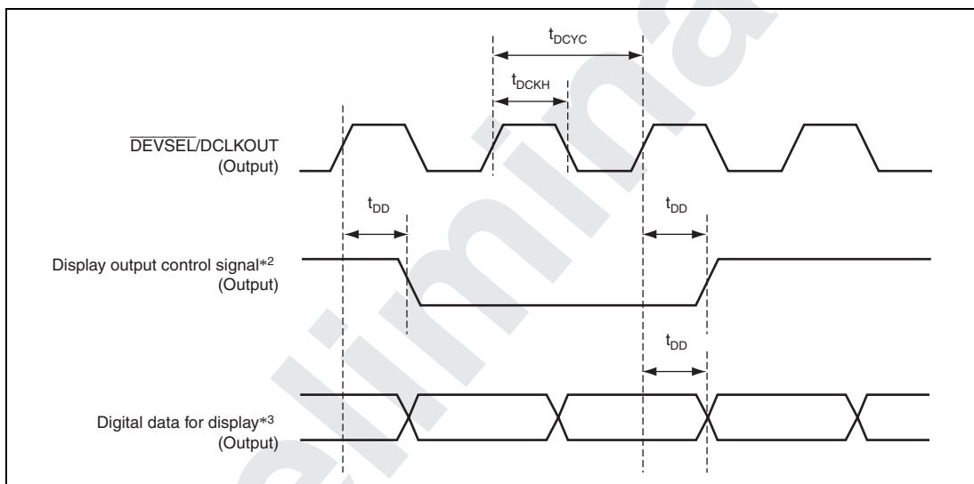
Figure 32.75 Display Timing (with Respect to \overline{DEVSEL}/DCLKOUT )
