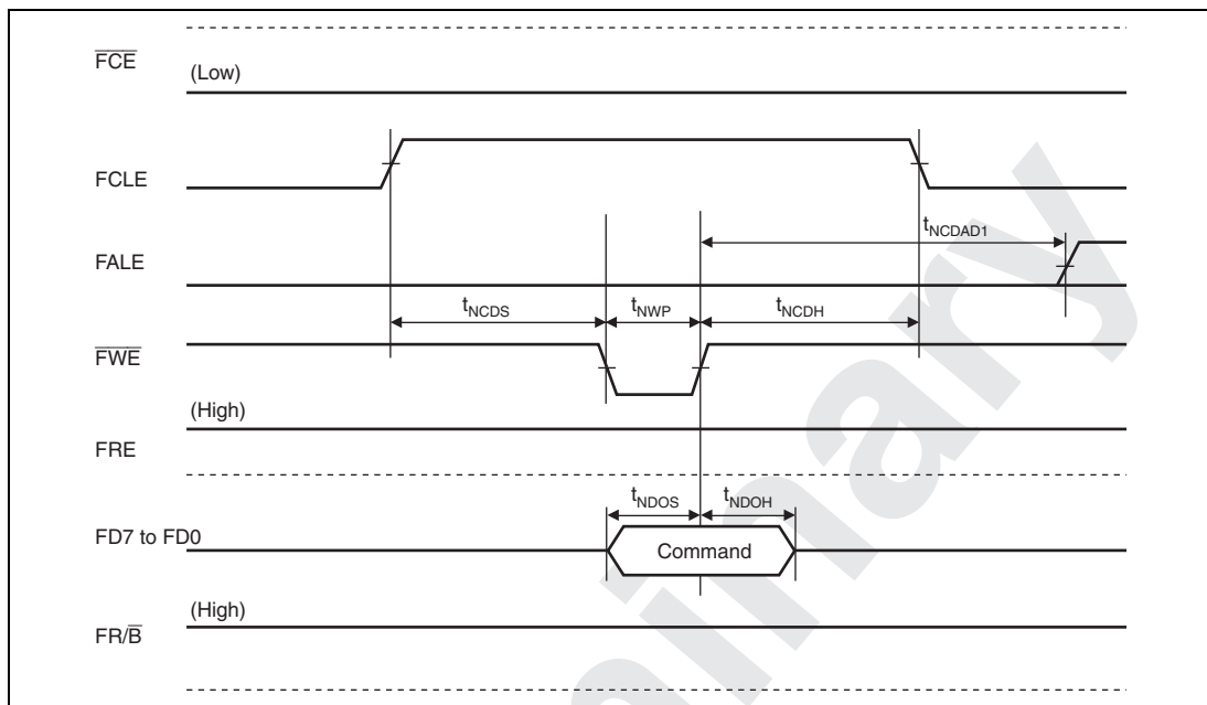
Figure 32.68 Command Issue Timing of NAND-Type Flash Memory
