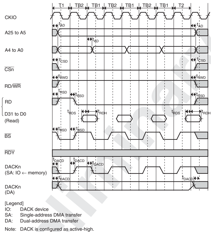
Figure 32.13 Burst ROM Bus Cycle (No Wait)
