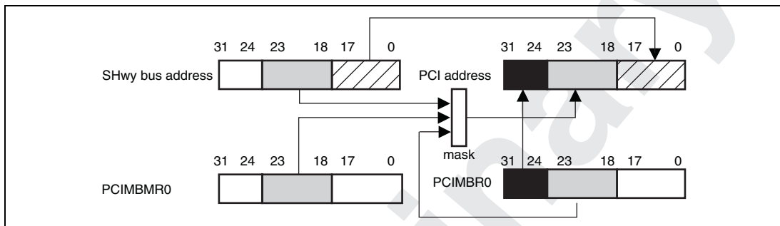
Figure 13.3 Access from SHwy Bus to PCI Memory (PCI Bus) (PCI Memory Space 0)
