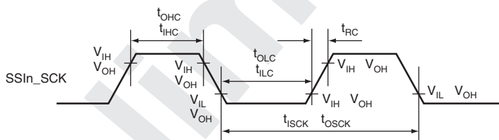
Figure 32.63 SSI Clock Input/Output Timing
