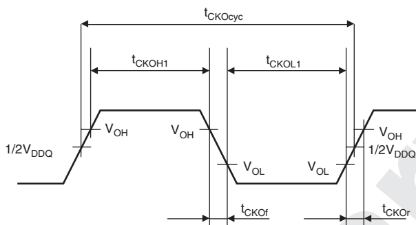
Figure 32.2 CLKOUT Clock Output Timing (1)
