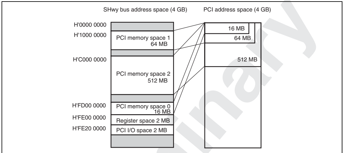
Figure 13.2 Memory Map from SHwy Bus to PCI Bus
