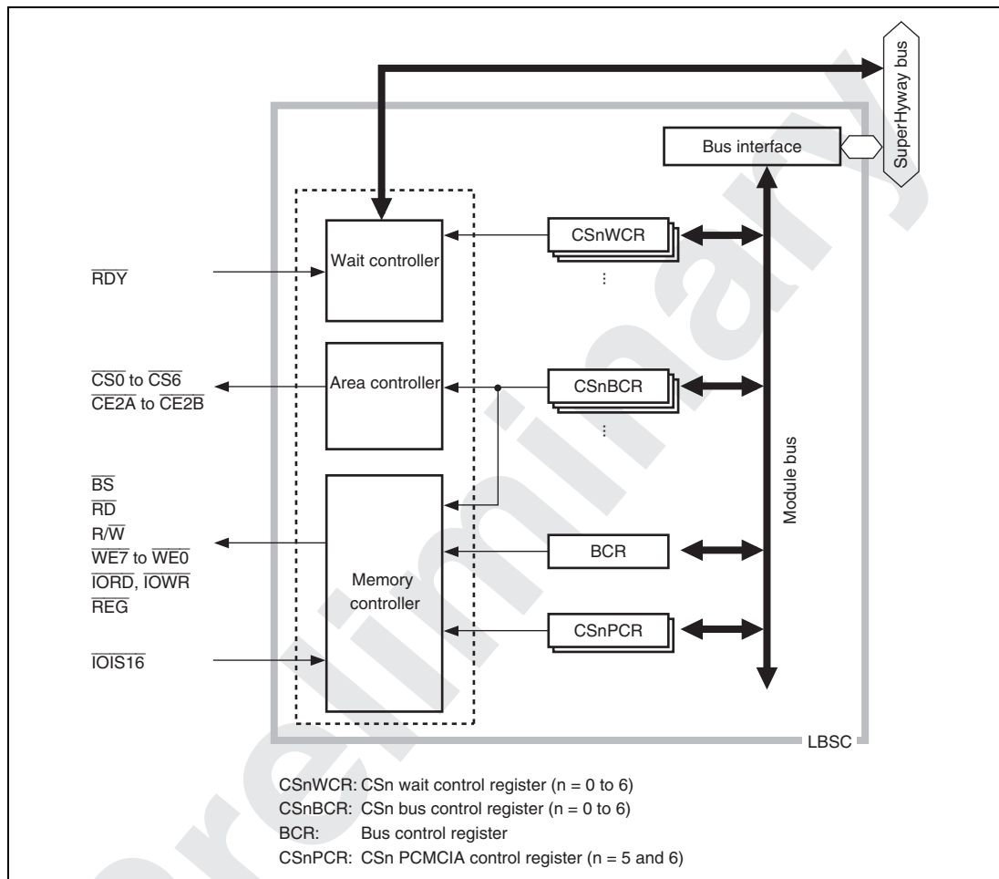
Figure 11.1 Block Diagram of LBSC
