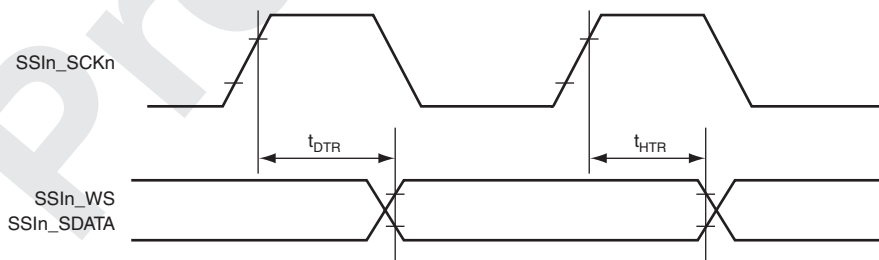
Figure 32.64 SSI Transmission Timing (1)
