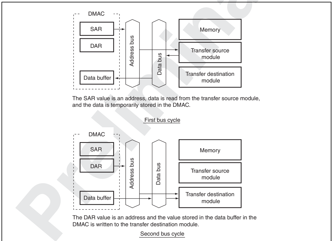
Figure 14.4 Data Flow of Dual Address Mode
