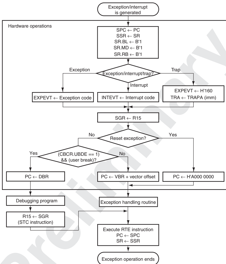
Figure 29.2 Flowchart of User Break Debugging Support Function
