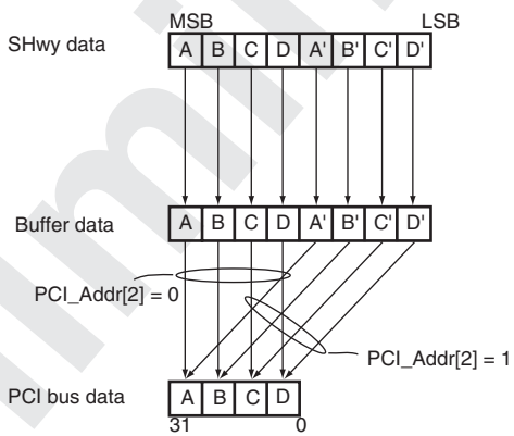
Figure 13.7 Endian Conversion from SHwY Bus to PCI Bus (Non-Byte Swapping: TBS = 0)
