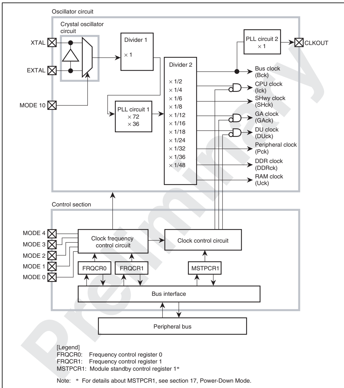
Figure 15.1 Block Diagram of the CPG
