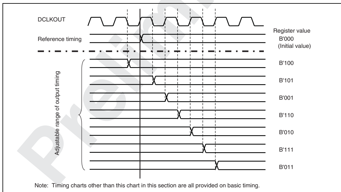
Figure 19.19 Adjustable Range of Output Timing
