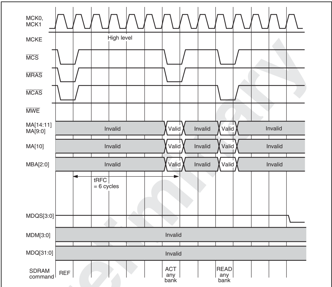
Figure 12.20 t_{RFC}
