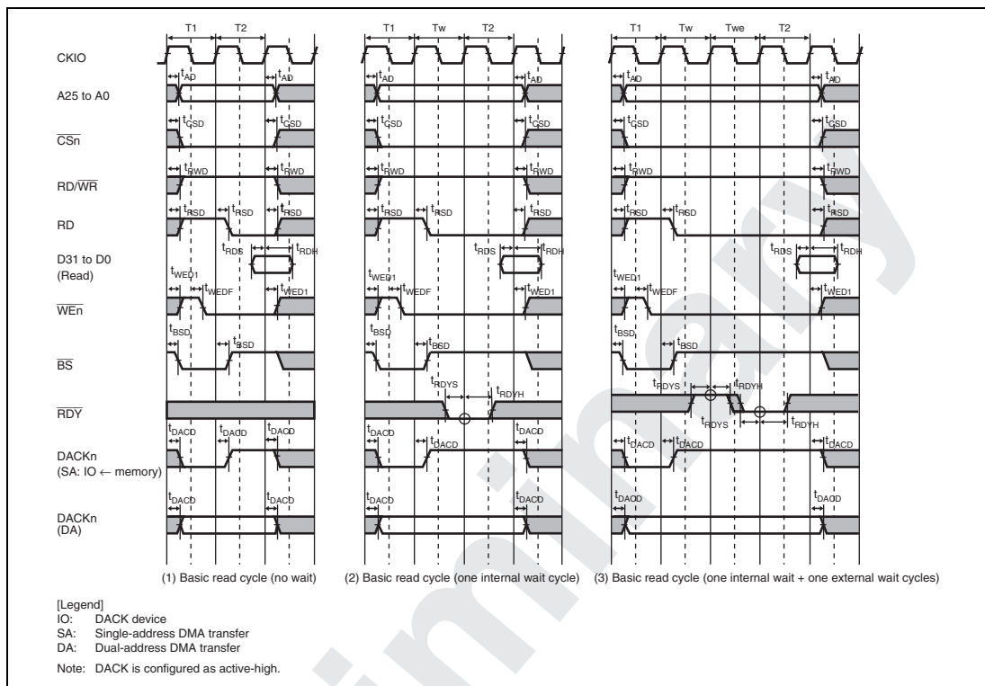
Figure 32.24 Memory Byte Control SRAM Bus Cycle
