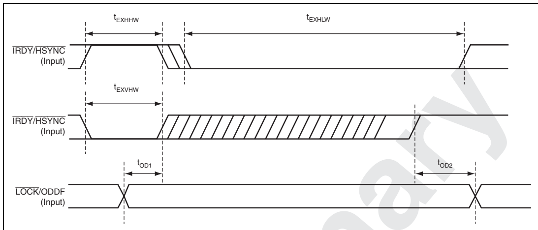
Figure 32.76 Display Timing in TV Synchronous Mode
