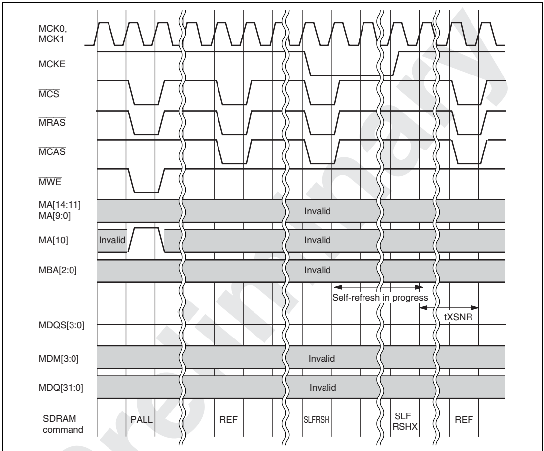
Figure 12.13 Self-Refresh Operation
