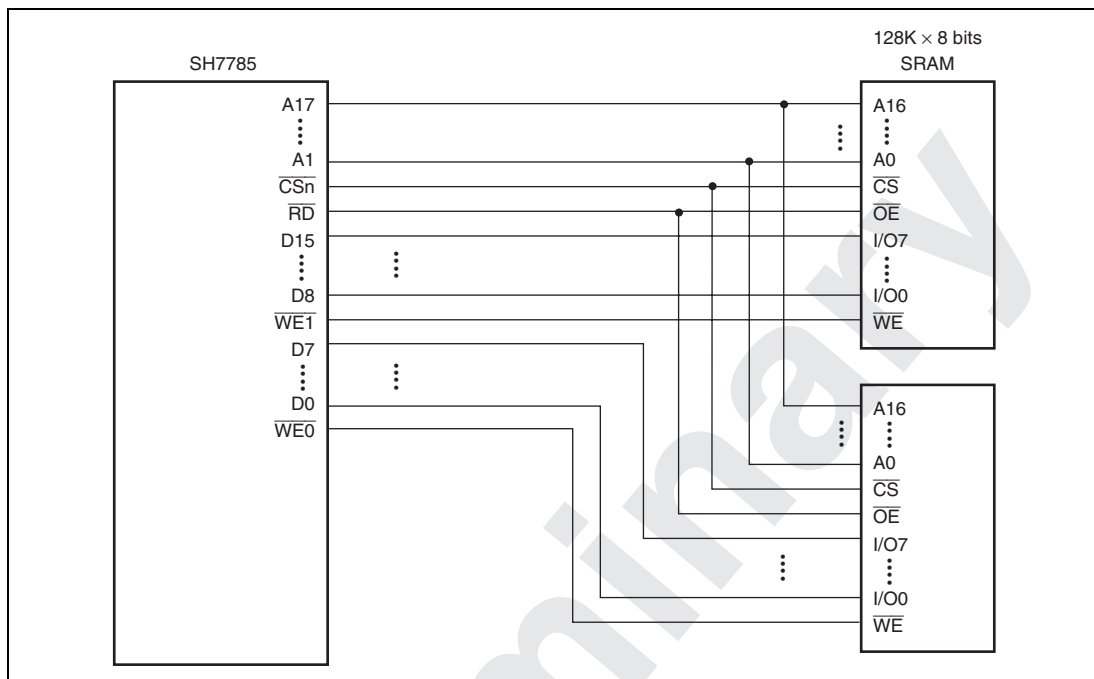
Figure 11.7 Example of 16-Bit Data Width SRAM Connection
