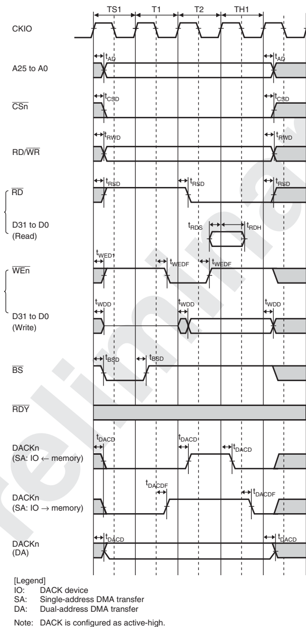
Figure 32.12 SRAM Bus Cycle: Basic Bus Cycle ( \overline{CSnWCR.IW} = 0000 , \overline{CSnWCR.RDS} = 001 , \overline{CSnWCR.WTS} = 001 , \overline{CSnWCR.RDH} = 001 , \overline{CSnWCR.WTH} = 001 )
