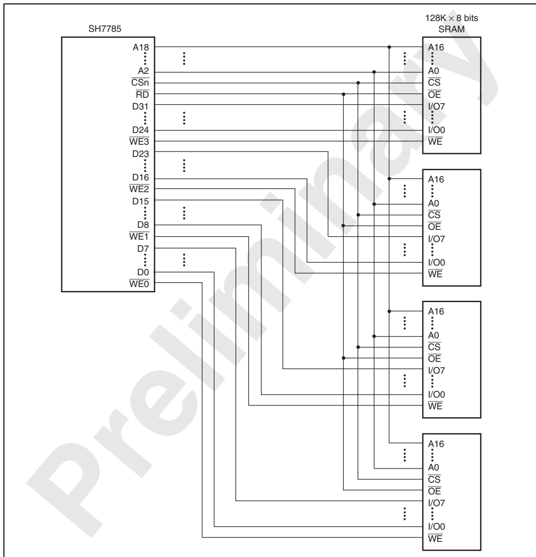
Figure 11.6 Example of 32-Bit Data Width SRAM Connection
