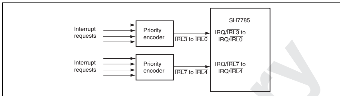
Figure 10.3 Example of IRL Interrupt Connection
