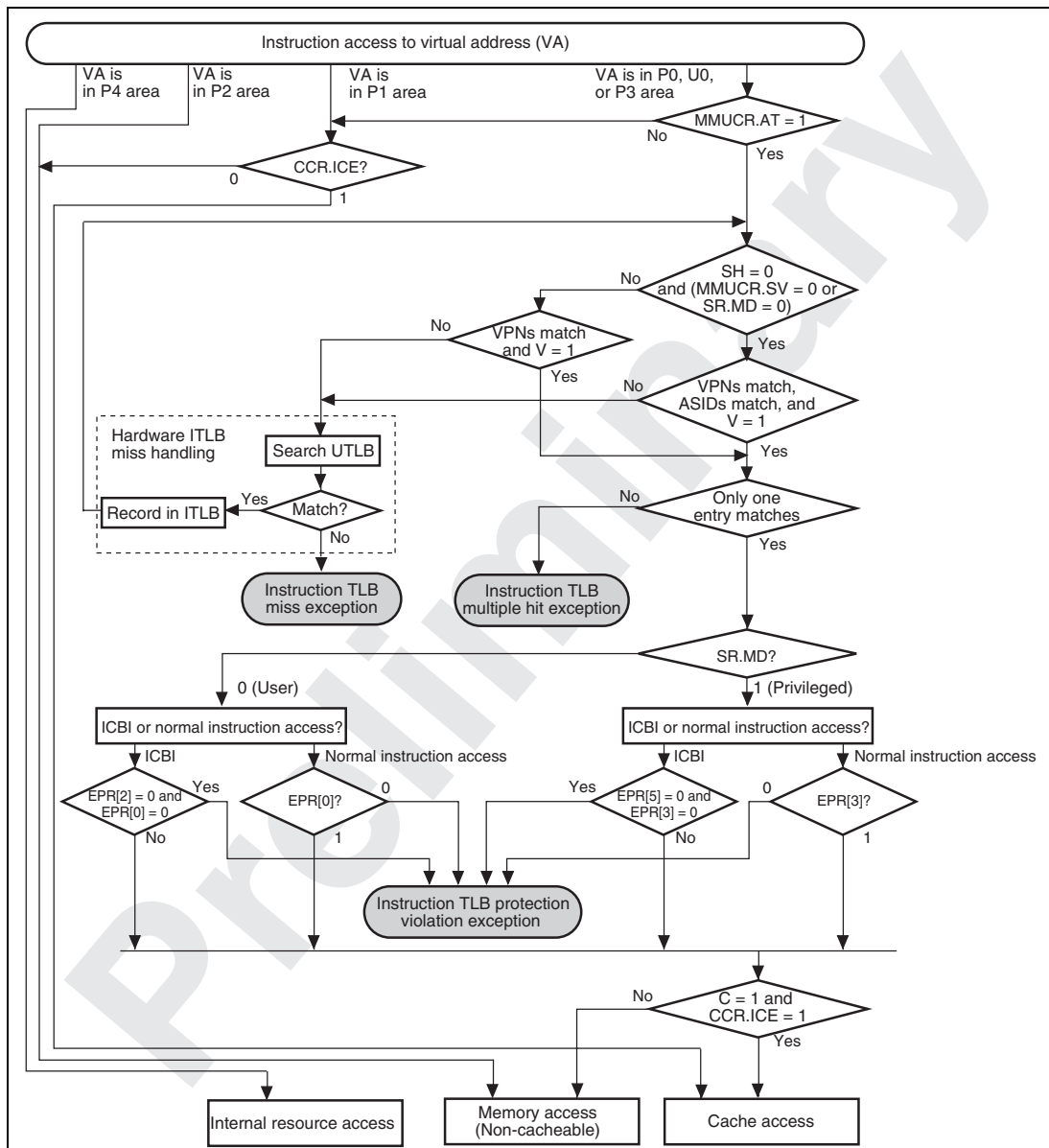
Figure D.7 Flowchart of Memory Access Using ITLB (TLB Extended Mode)
