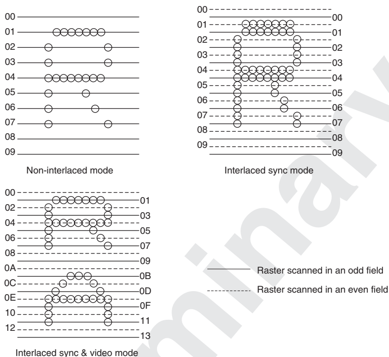
Figure 19.16 Example of Display in Each Scan Mode
