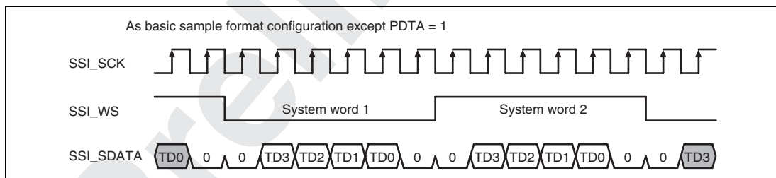
Figure 26.16 Parallel Right Aligned with Delay
