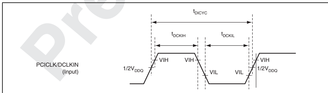
Figure 32.73 PCICLK/DCLKIN Clock Input Timing
