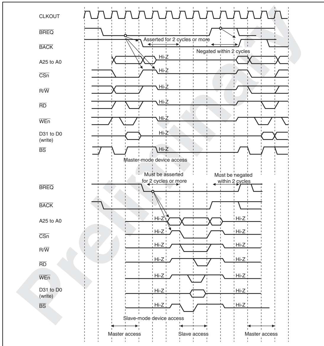
Figure 11.42 Arbitration Sequence
