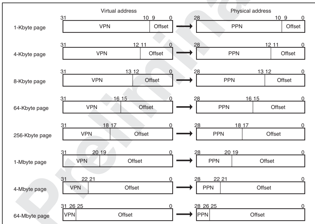
Figure D.4 Relationship between Page Size and Address Format (TLB Extended Mode)
