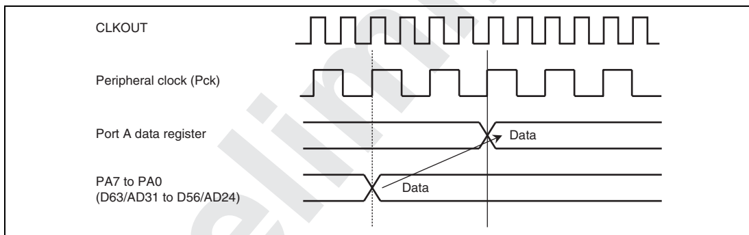
Figure 28.2 Port A Data Input Timing Diagram
