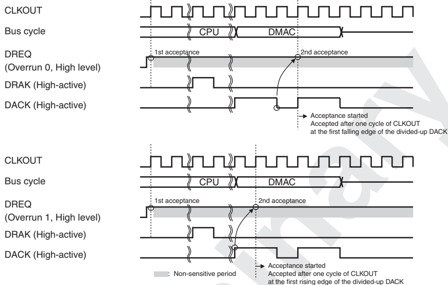
Figure 14.21 Example 2 of DREQ Input Detection in Burst Mode Level Detection (Word Transfer in 8-Bit Bus Width, Longword Transfer in 8/16-Bit Bus Width, 16/32-Byte Transfer in 8/16/32/64-Bit Bus Width: DACK of DMA1 Transfer Divided)
