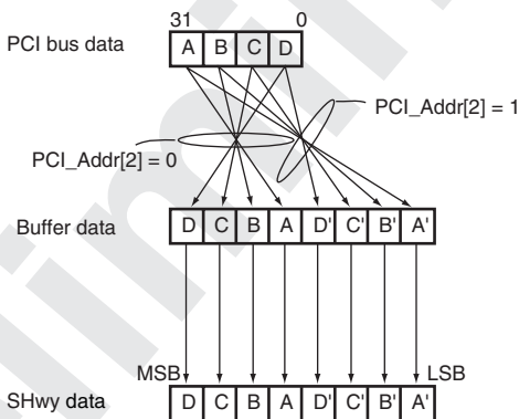
Figure 13.14 Endian Conversion from PCI Bus to SHwY Bus (Byte Swapping: TBS = 1)
