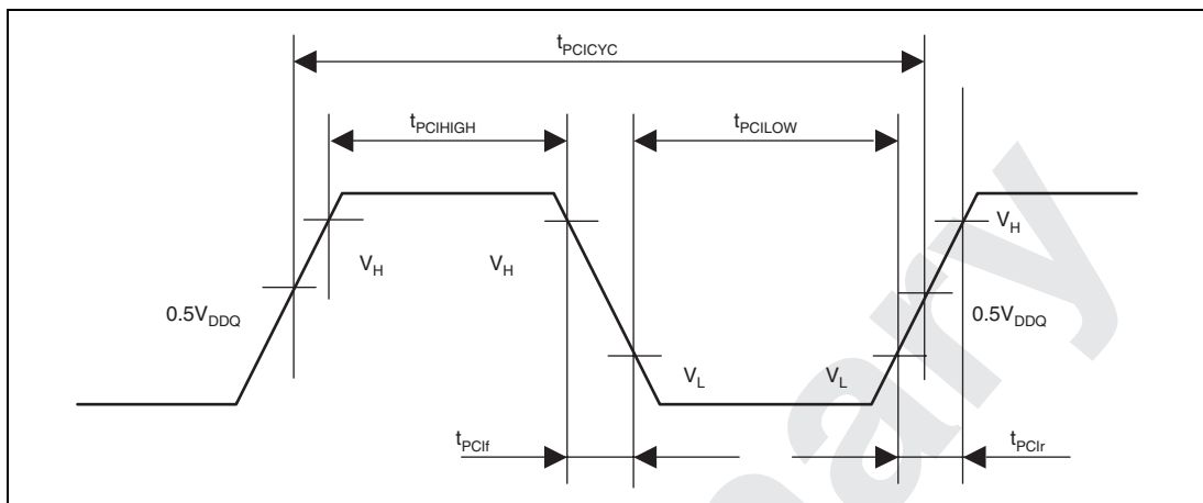
Figure 32.37 PCI Clock Input Timing
