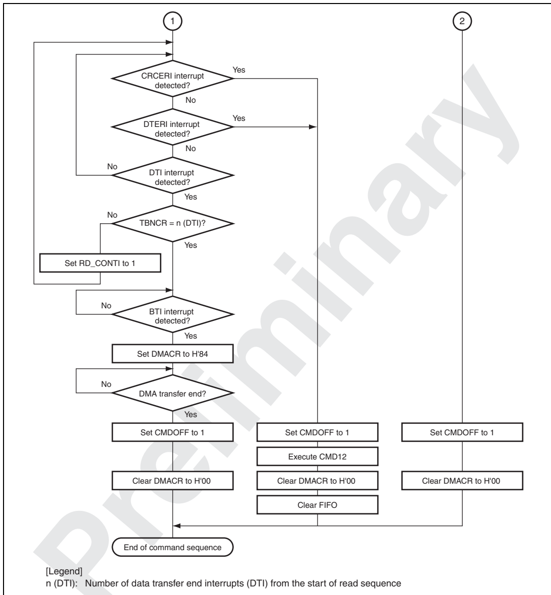
Figure 24.23 (4) Example of Read Sequence Flow (Pre-defined Multiple Block Transfer)
