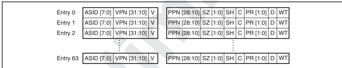
Figure 7.6 UTLB Configuration
