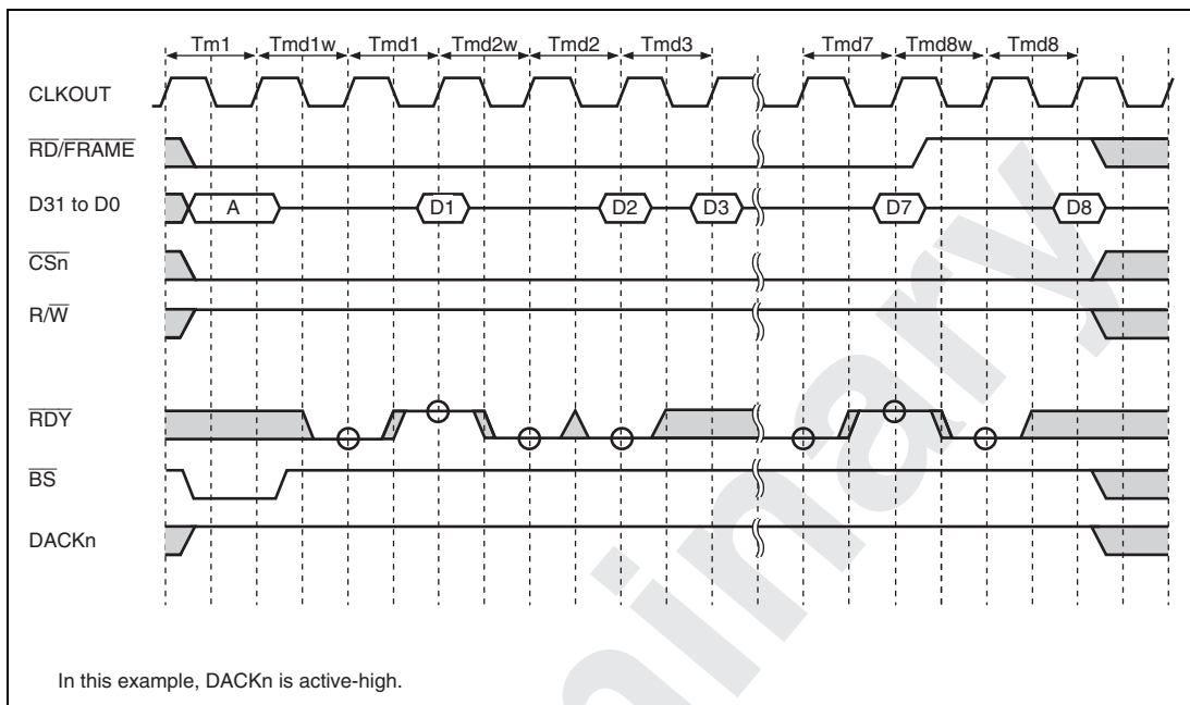
Figure 11.33 MPX Interface Timing 10 (Burst Read Cycle, IW = 0000, External Wait Control, 32-Bit Bus Width, 32-Byte Data Transfer)
