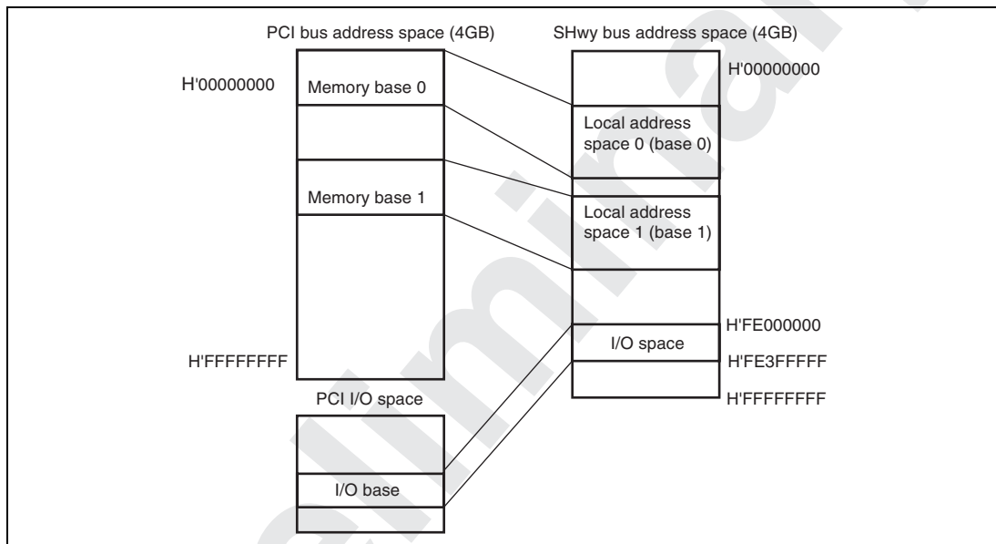
Figure 13.10 Memory Map from PCI Bus to SHwY Bus
