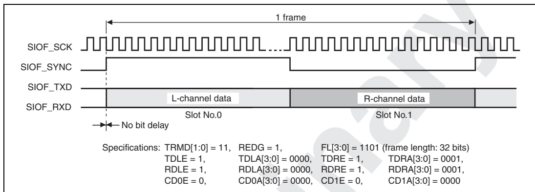
Figure 22.16 Transmit and Receive Timing (16-Bit Stereo Data (1))
