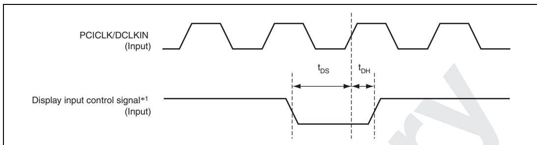
Figure 32.74 Display Timing (with Respect to PCICLK/DCLKIN)
