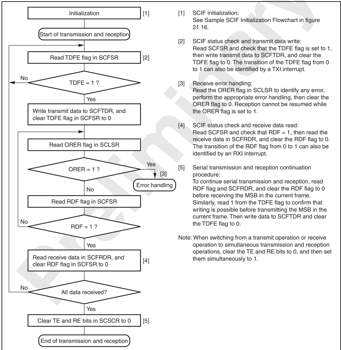
Figure 21.21 Sample Flowchart for Transmitting/Receiving Serial Data
