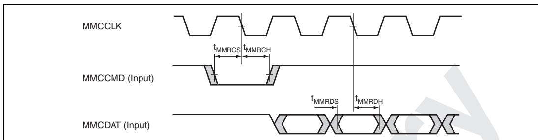
Figure 32.58 MMCIF Reception Timing (Sampling on Falling Edges)
