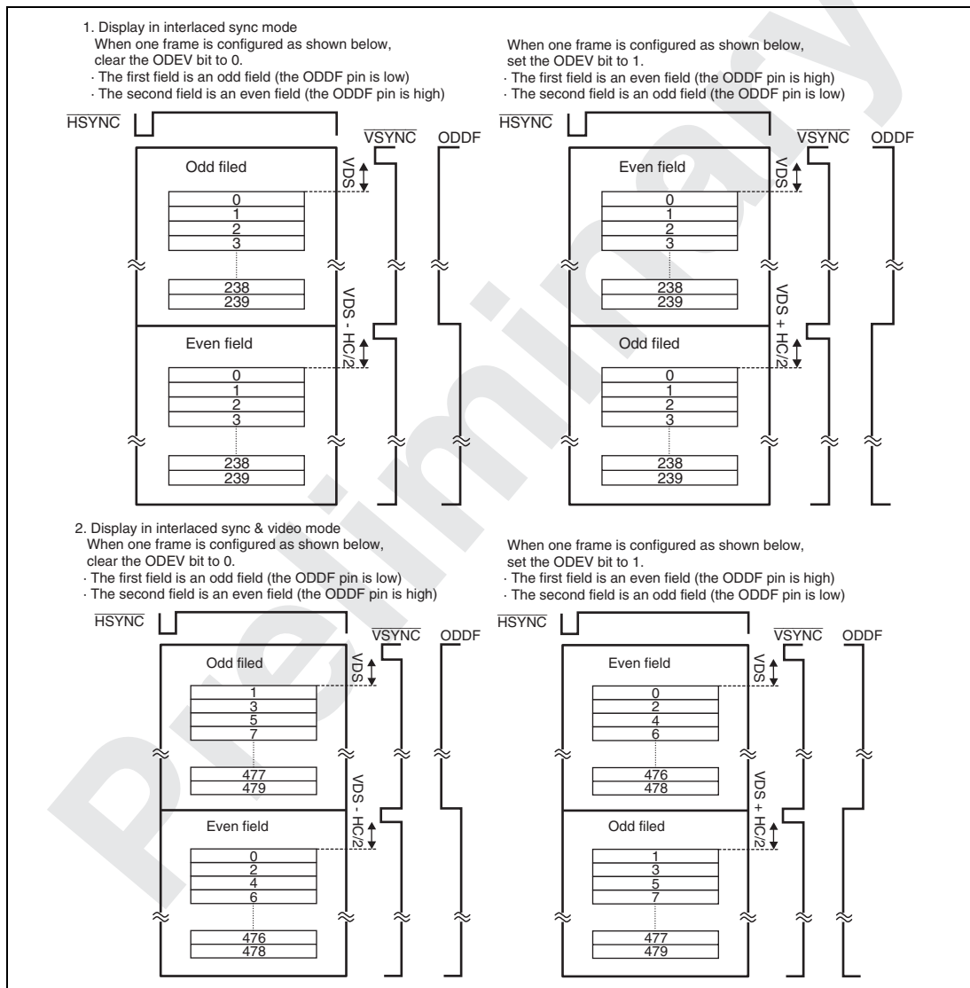
Figure 19.18 Display in Interlaced Method
