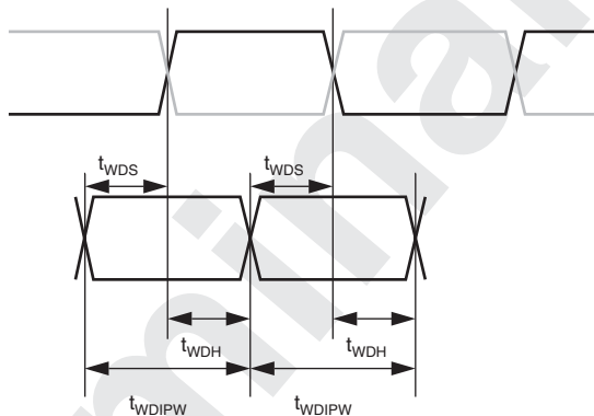
Figure 32.32 MDQS and MDQ/MDM Output Waveform (Write)
