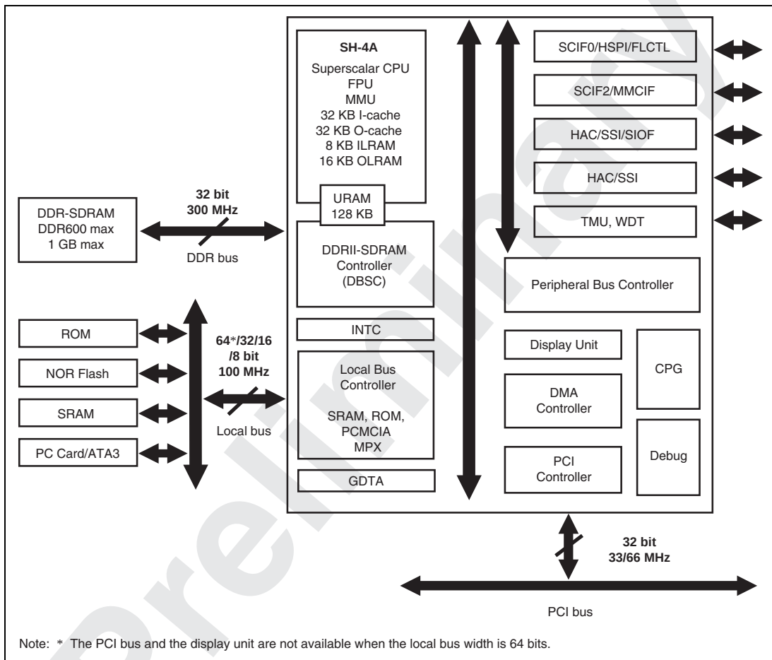
Figure 1.1 SH7785 Block Diagram
