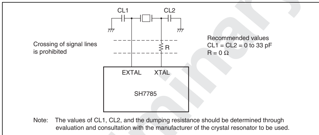
Figure 15.4 Note on Using a Crystal Resonator
