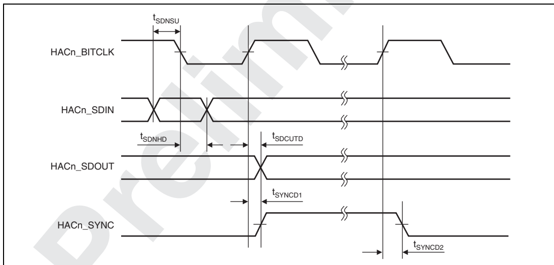
Figure 32.62 HAC Interface Module Signal Timing
