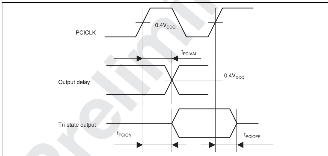
Figure 32.38 PCI Output Signal Timing
