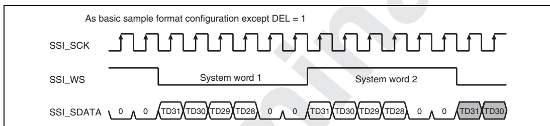
Figure 26.15 Serial Data First, Followed by Padding Bits, without Delay
