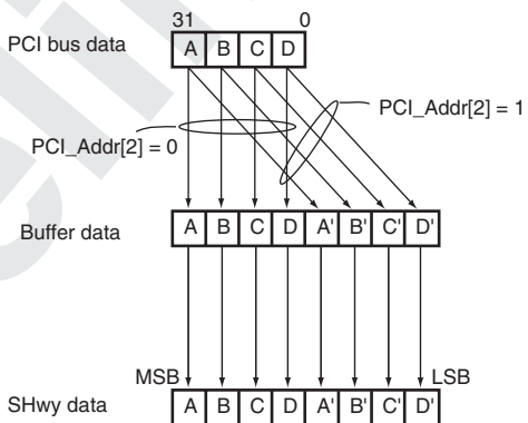
Figure 13.13 Endian Conversion from PCI Bus to SHwY Bus (Non-Byte Swapping: TBS = 0)
