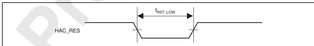
Figure 32.59 HAC Cold Reset Timing
