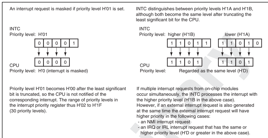
Figure 10.4 Priority of On-Chip Peripheral Module Interrupts
