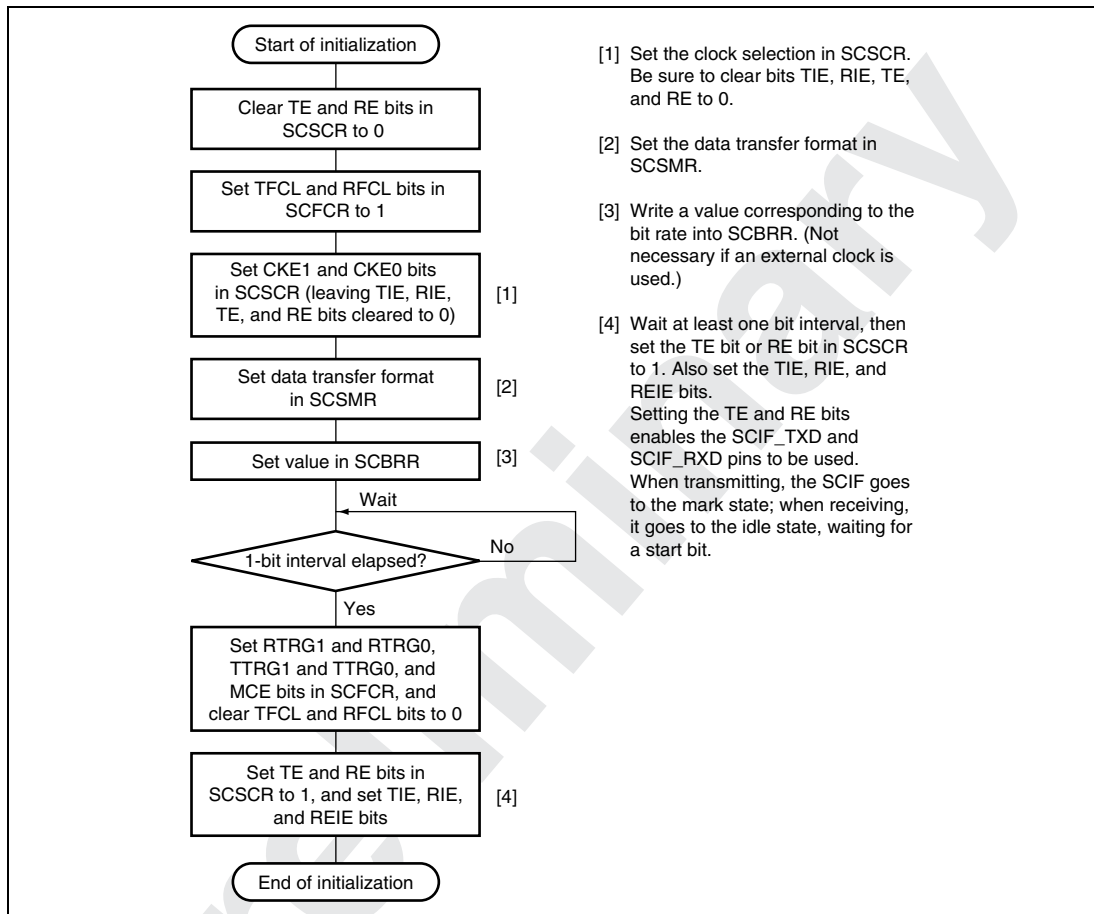
Figure 21.8 Sample SCIF Initialization Flowchart
