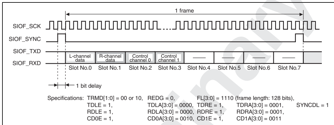
Figure 22.18 Transmit and Receive Timing (16-Bit Stereo Data (3))
