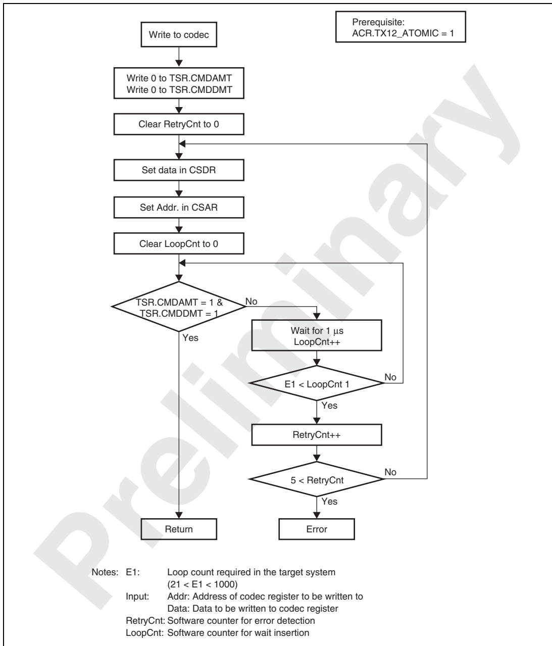
Figure 25.4 Sample Flowchart for Off-Chip Codec Register Write
