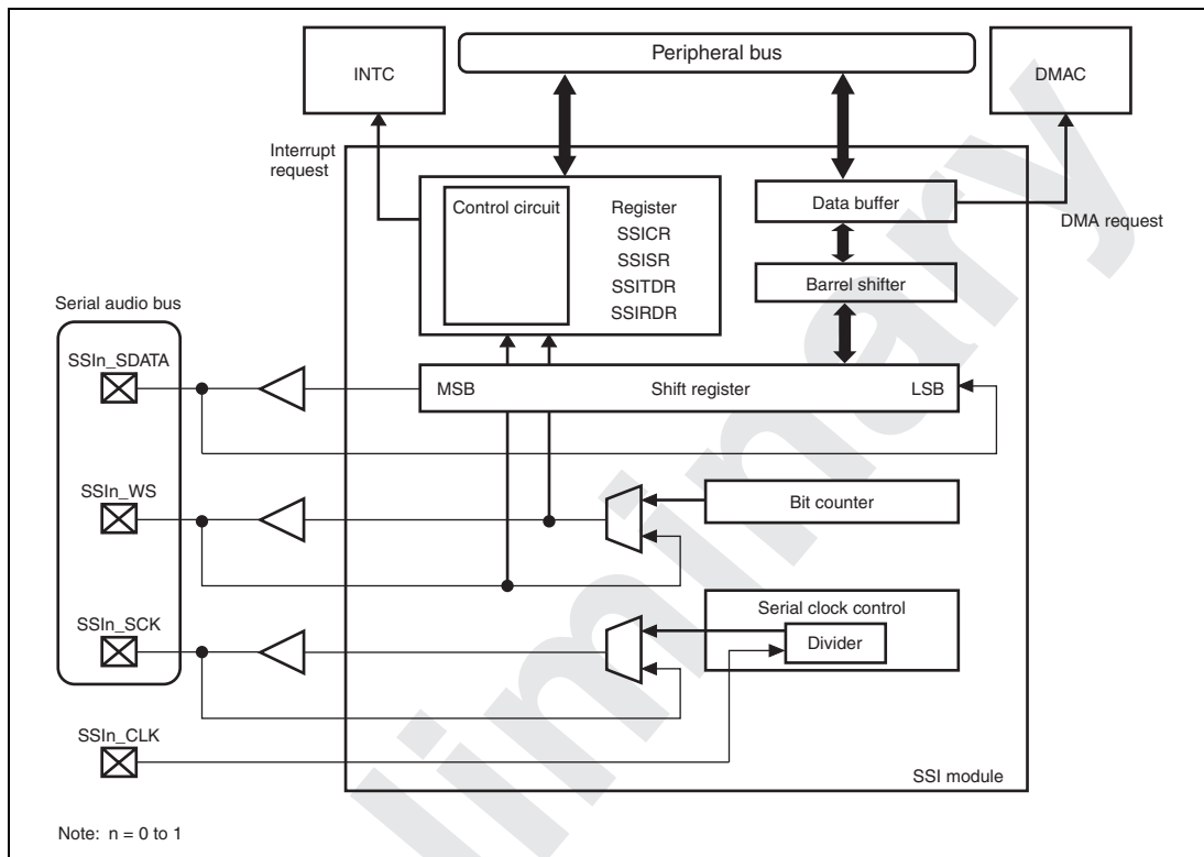
Figure 26.1 Block Diagram of SSI Module
