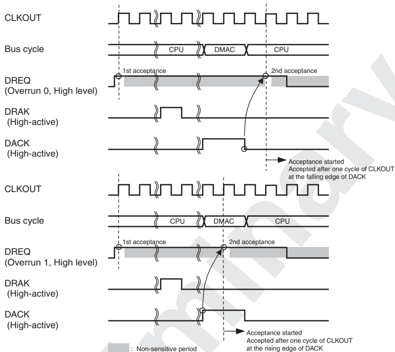
Figure 14.16 Example 1 of DREQ Input Detection in Cycle Steal Mode Level Detection (Byte Transfer in 8/16/32/64-Bit Bus Width, Word Transfer in 16/32/64-Bit Bus Width, or Longword Transfer in 32/64-Bit Bus Width)
