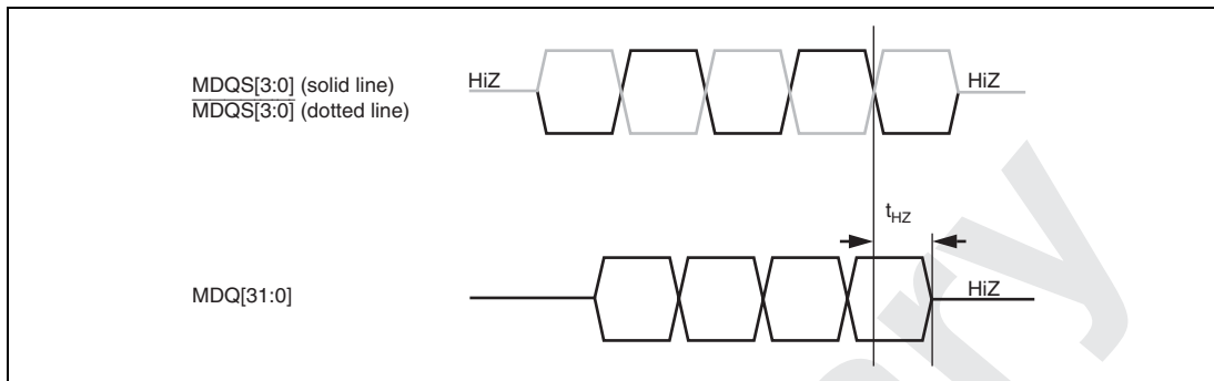
Figure 32.33 MDQ high-impedance time from MDQS (Write)
