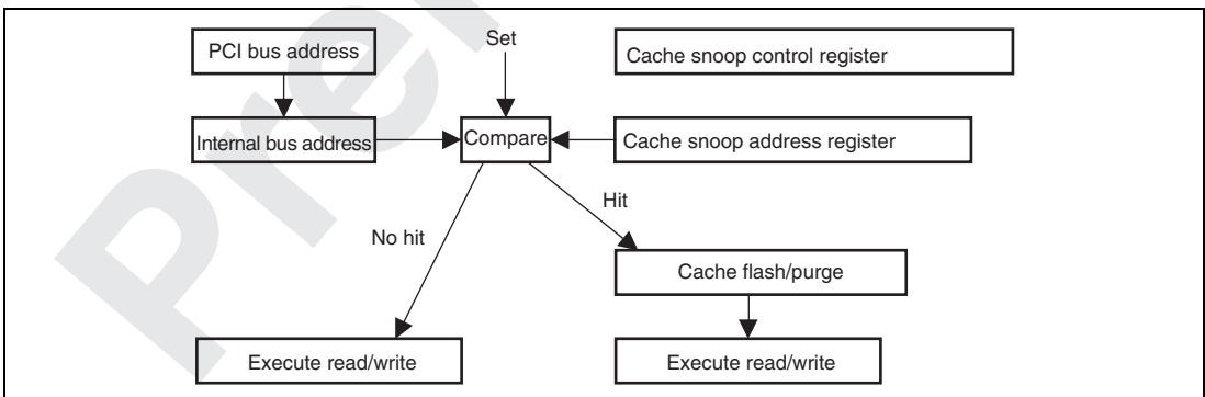
Figure 13.16 Cache Flash/Purge Execution Flow from PCI Bus to SHwy Bus
