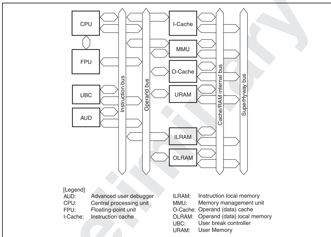
Figure D.1 Block Diagram
