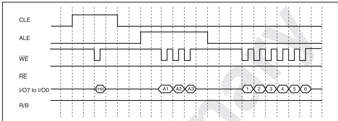
Figure 27.3 Writing Operation Timing for NAND-Type Flash Memory
