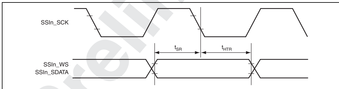
Figure 32.67 SSI Reception Timing (2)
