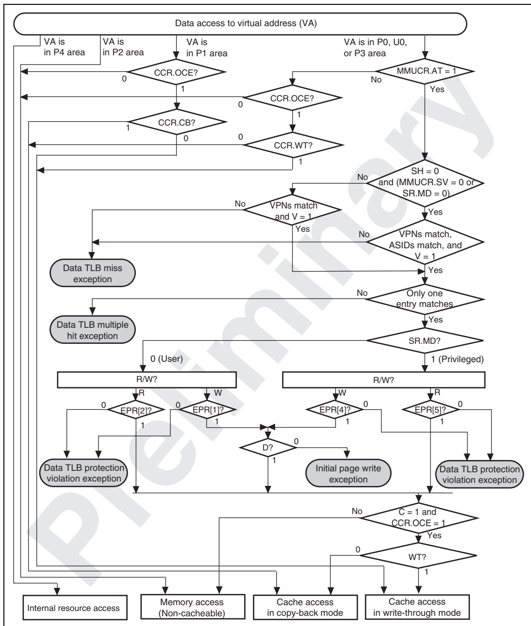
Figure D.6 Flowchart of Memory Access Using UTLB (TLB Extended Mode)
