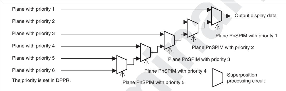
Figure 19.5 Plane Processing Sequence in α Blending and EOR Operation
