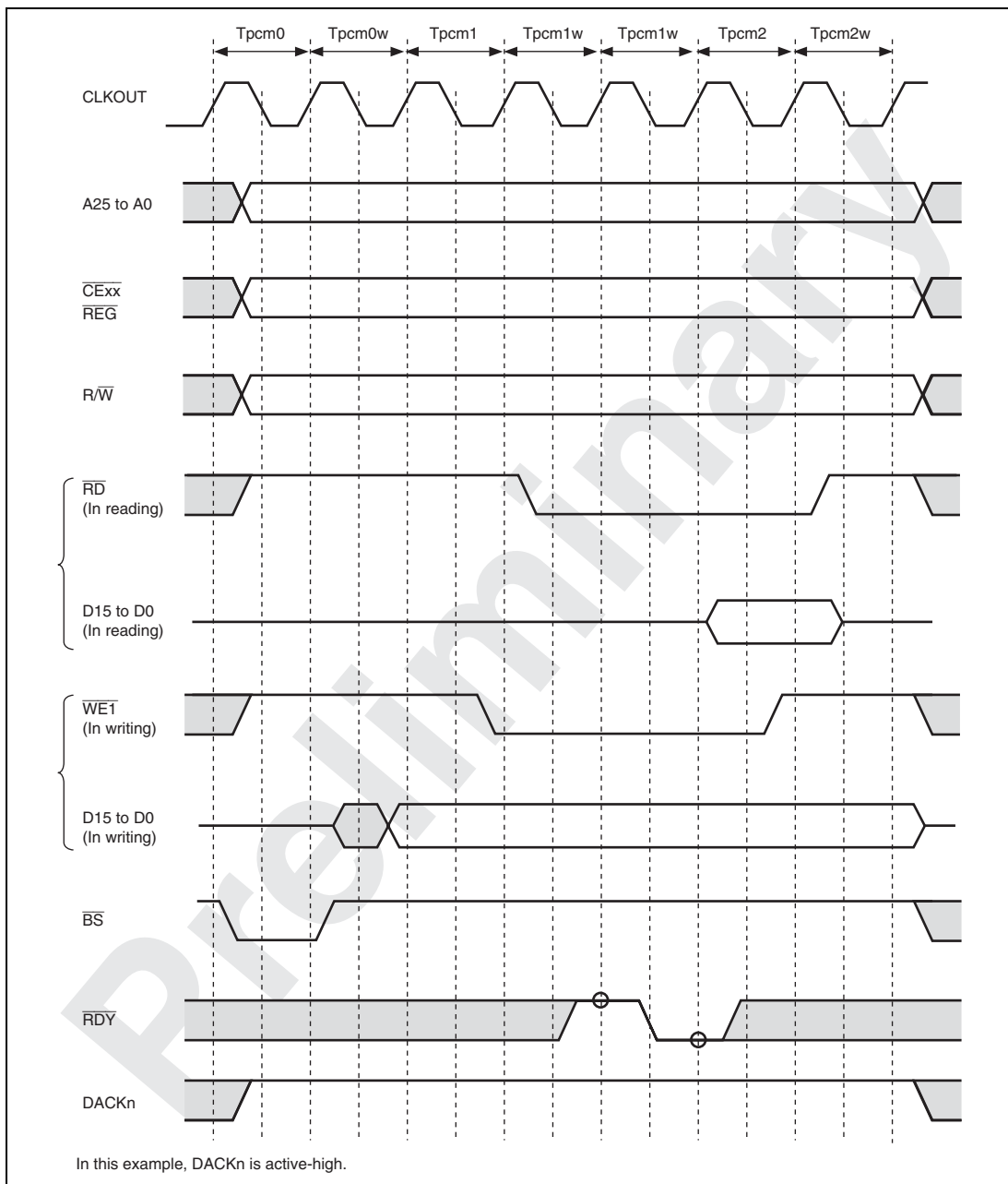
Figure 11.18 Wait Timing for PCMCIA Memory Card Interface
