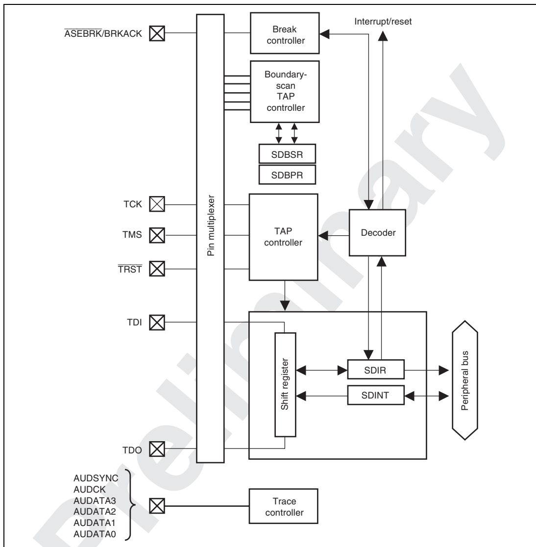
Figure 30.1 Block Diagram of H-UDI
