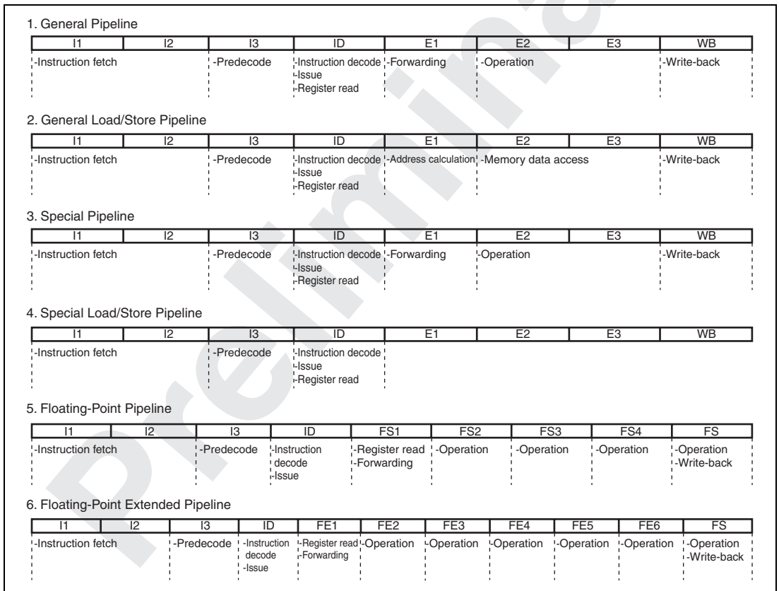
Figure D.2 Basic Pipelines
