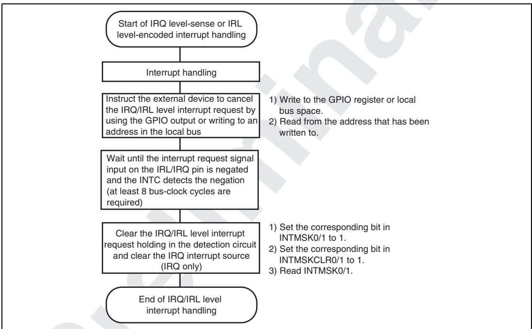
Figure 10.6 Example of Interrupt Handling Routine
