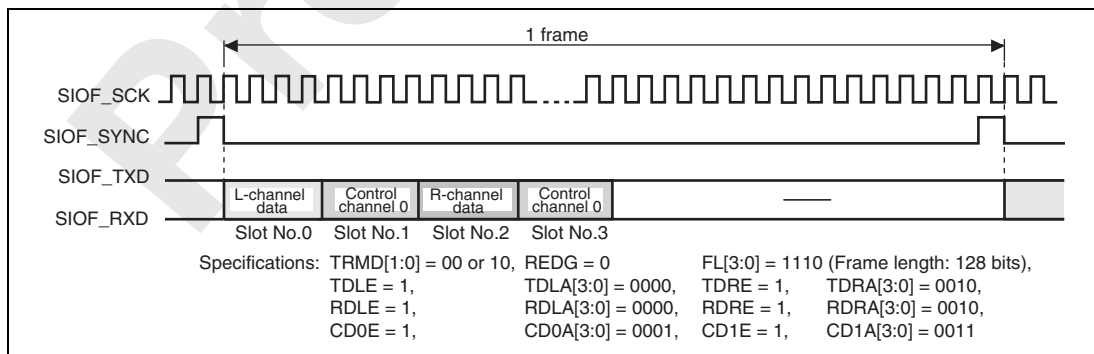
Figure 22.7 Control Data Interface (Slot Position)
