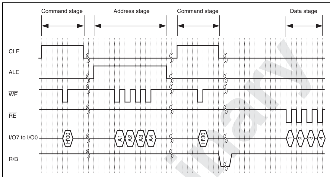
Figure 27.5 Reading Operation Timing for NAND-Type Flash Memory
