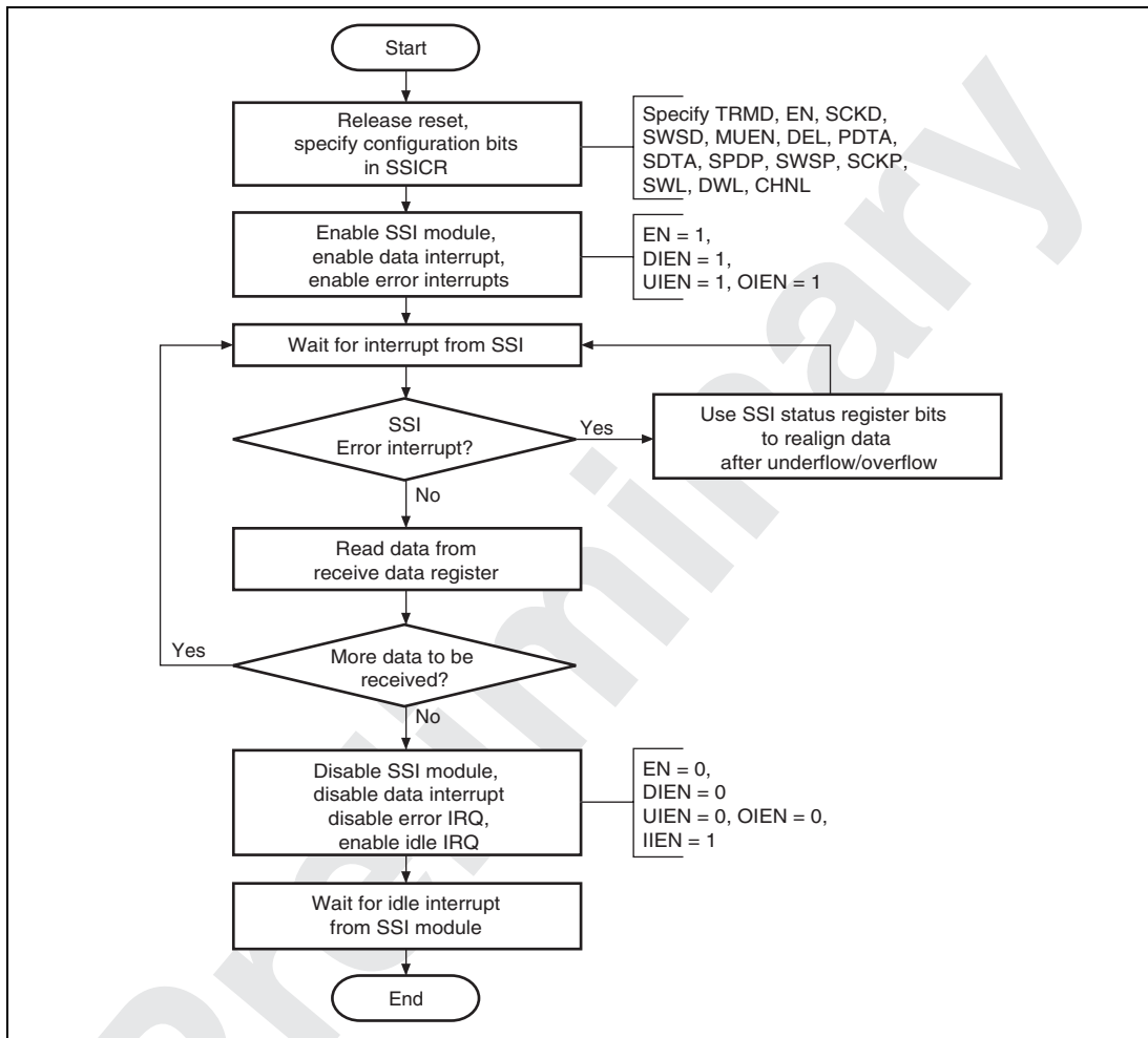
Figure 26.24 Reception using Interrupt Data Flow Control
