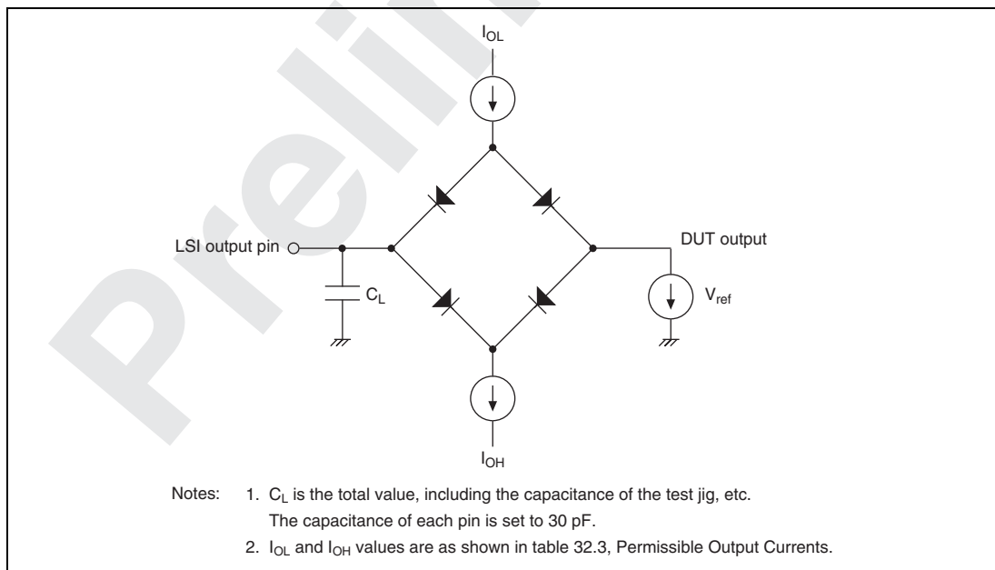
Figure 32.77 Output Load Circuit
