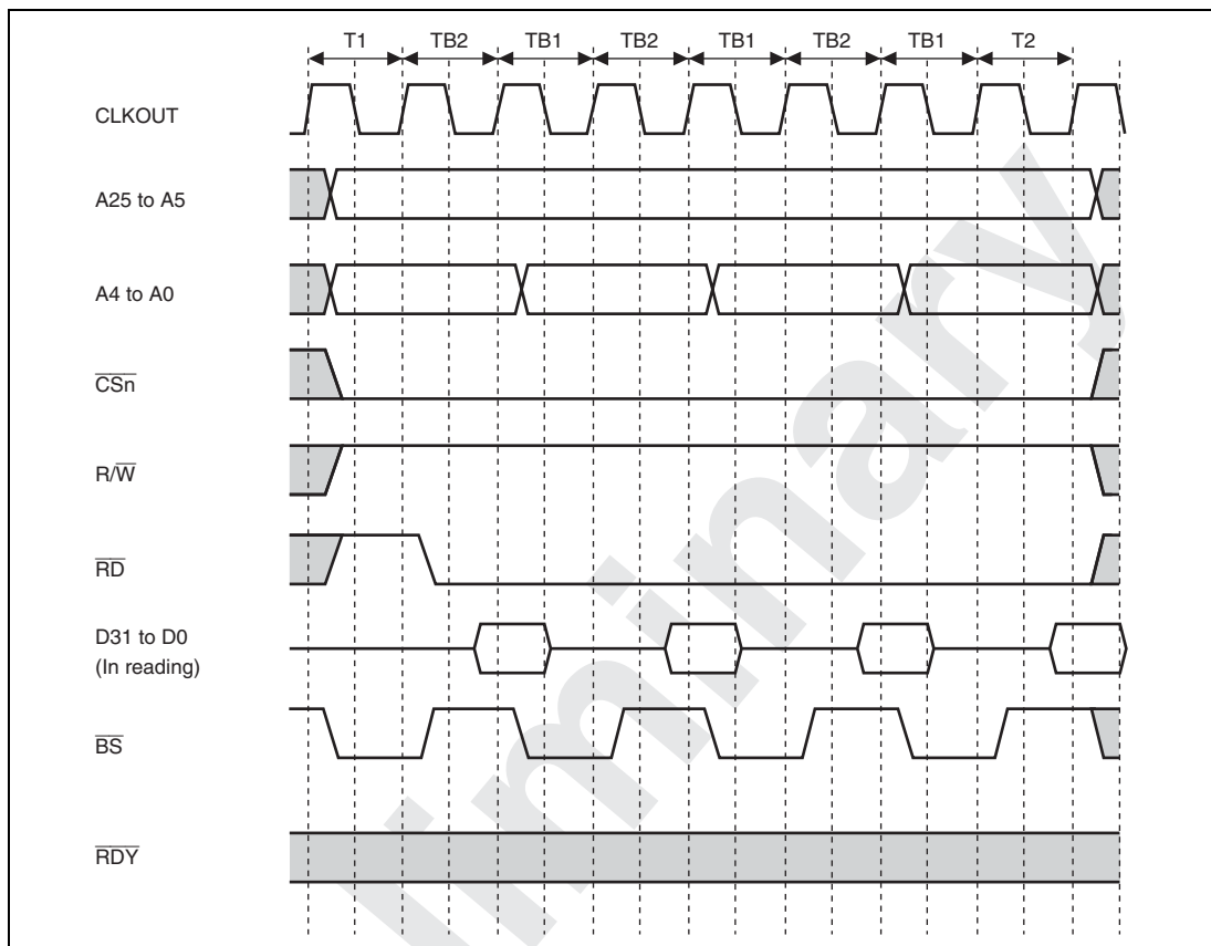
Figure 11.12 Burst ROM Basic Timing
