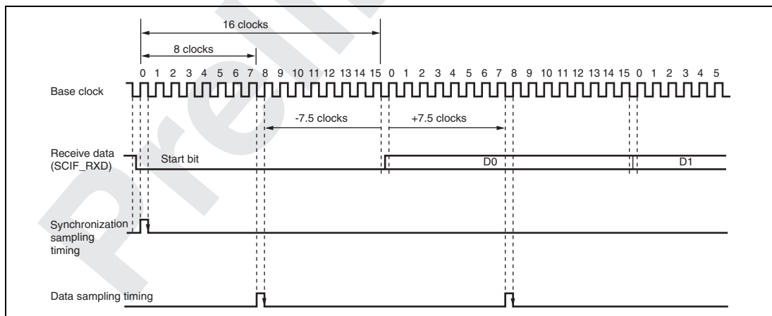
Figure 21.22 Receive Data Sampling Timing in Asynchronous Mode
