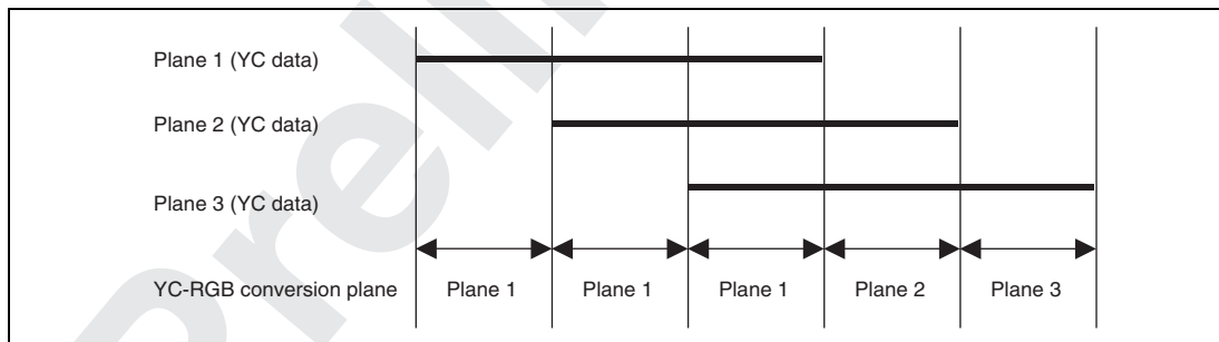
Figure 19.8 YC Data Contention
