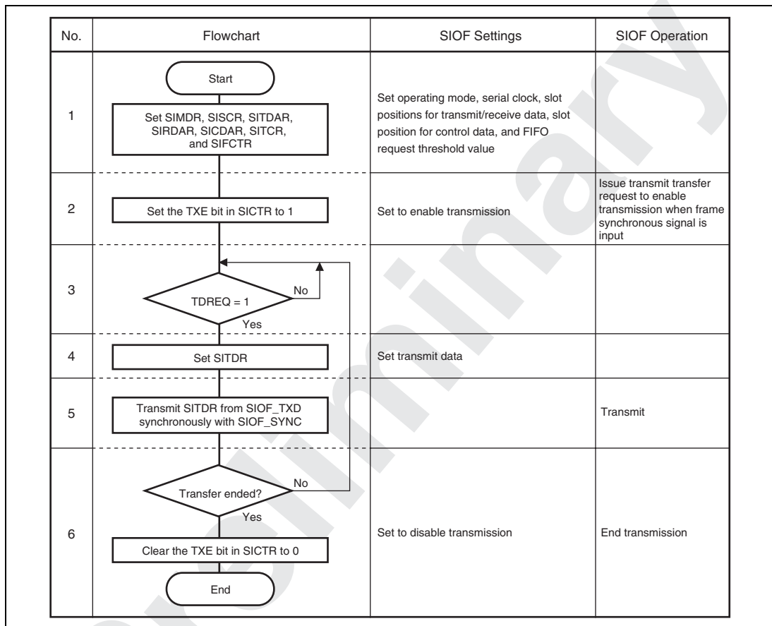
Figure 22.11 Example of Transmit Operation in Slave Mode
