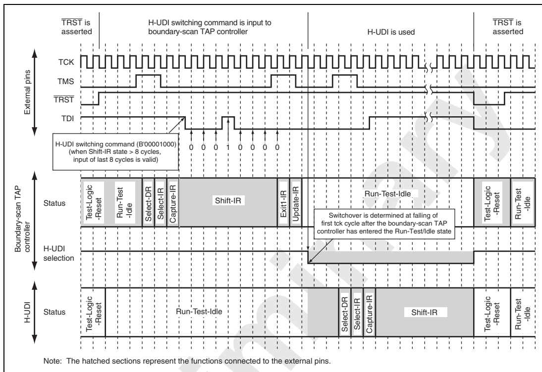
Figure 30.2 Sequence to Switch from Boundary-Scan TAP Controller to H-UDI
