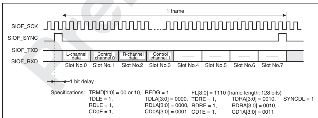
Figure 22.19 Transmit and Receive Timing (16-Bit Stereo Data (4))
