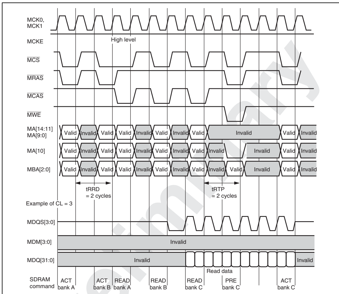
Figure 12.15 t_{RRD} and t_{RTP}
