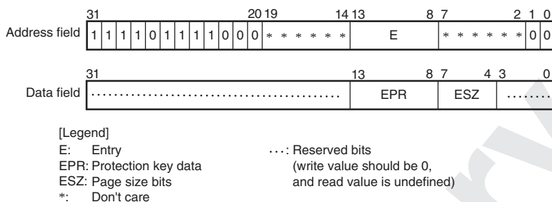
Figure D.12 Memory-Mapped UTLB Data Array 2 (TLB Extended Mode)
