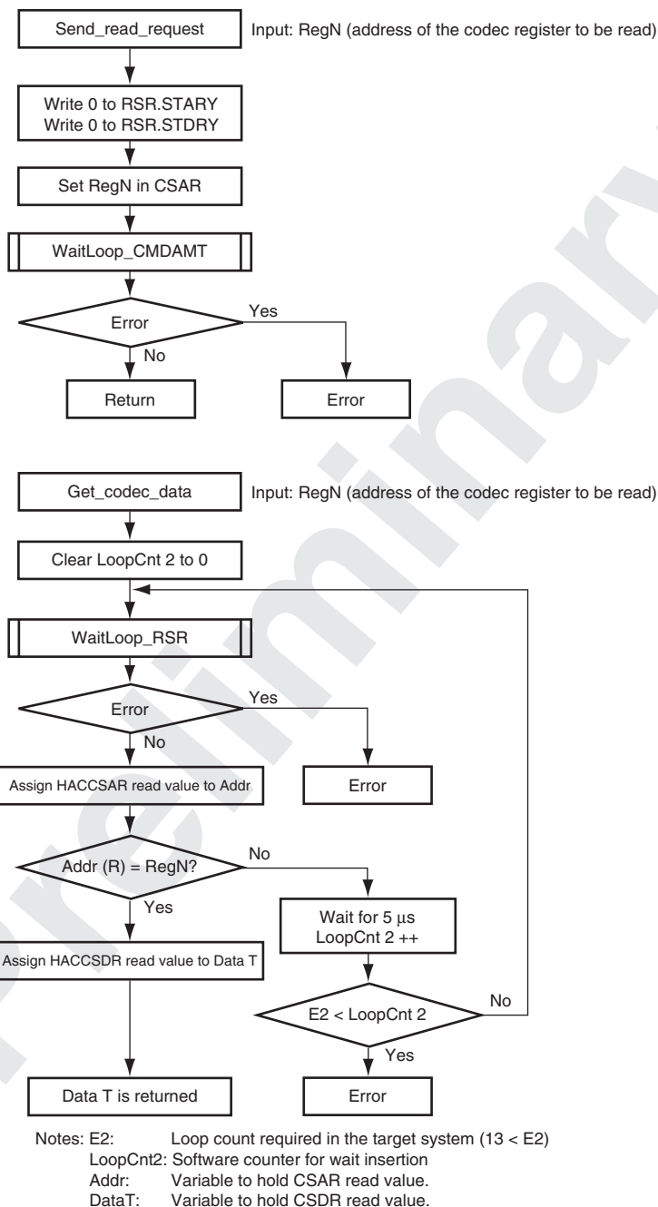
Figure 25.6 Sample Flowchart for Off-Chip Codec Register Read (2)
