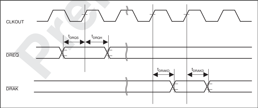
Figure 32.40 \overline{DREQ}/\overline{DRAK} Signal Timing
