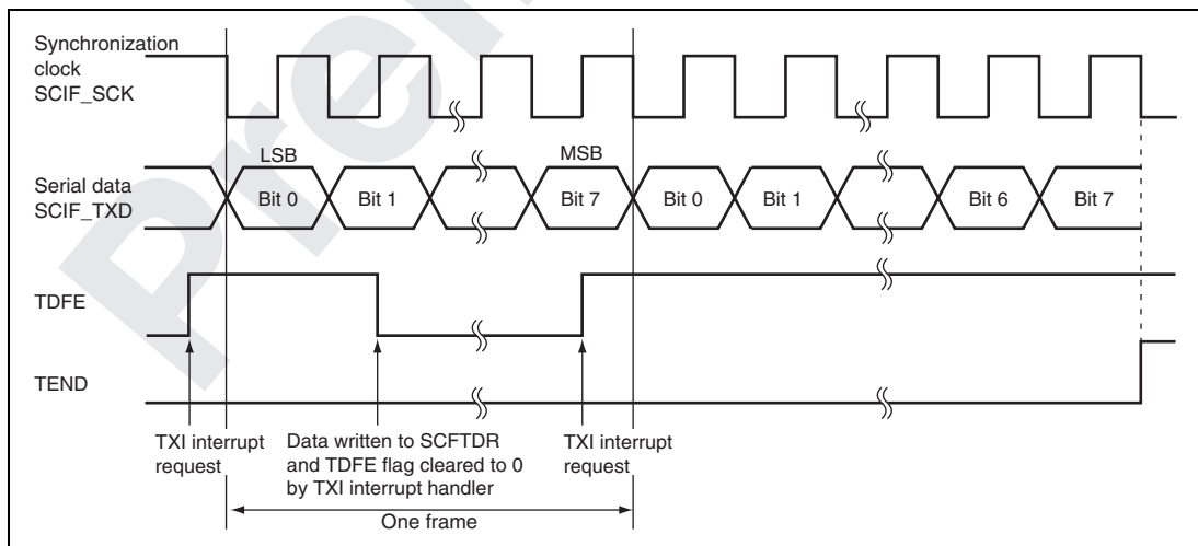
Figure 21.18 Example of SCIF Transmission Operation
