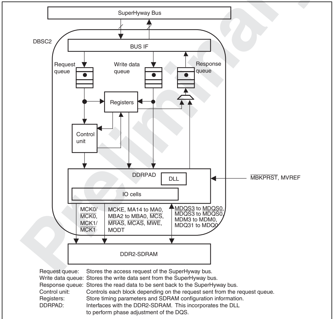
Figure 12.1 Block Diagram of the DBSC2
