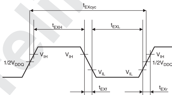
Figure 32.1 EXTAL Clock Input Timing
