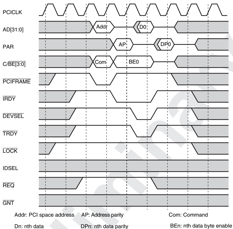
Figure 13.20 Master Read Cycle in Host Mode (Single)
