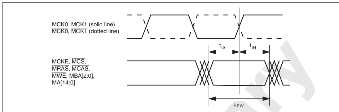
Figure 32.27 Command Signal and MCK Output Clock
