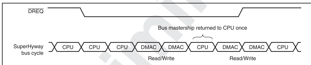
Figure 14.6 DMA Transfer Timing Example in Cycle Steal Normal Mode 1 (DREQ Low Level Detection)
