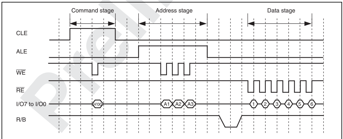
Figure 27.2 Reading Operation Timing for NAND-Type Flash Memory
