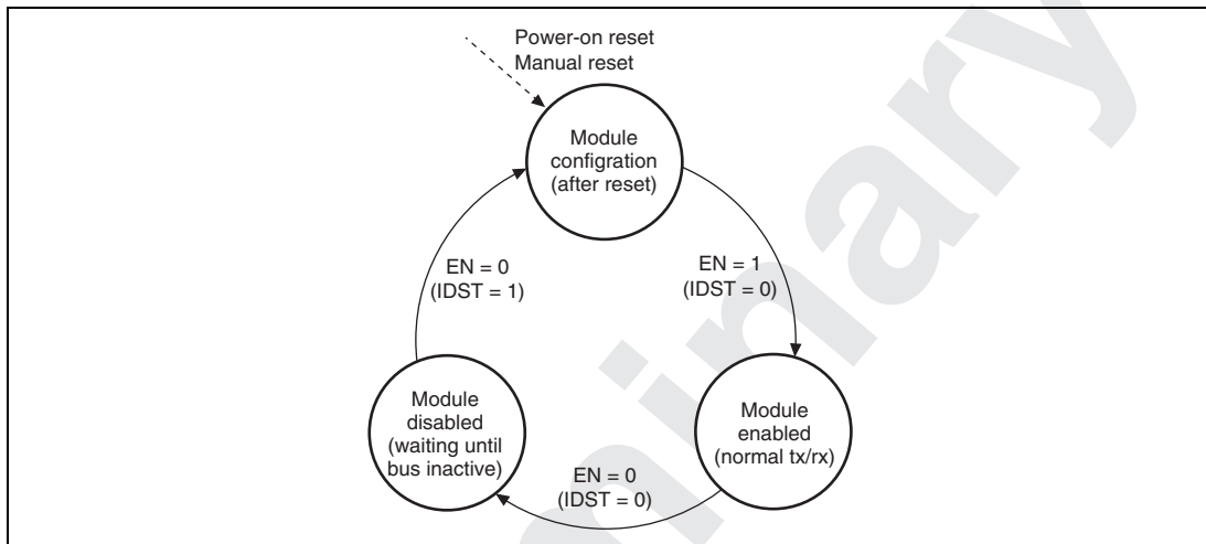
Figure 26.20 Transition Diagram between Operation Modes
