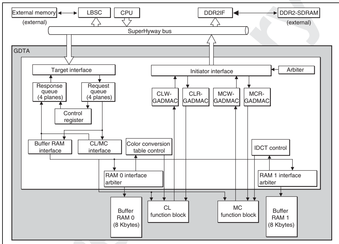
Figure 20.1 GDTA Block Diagram
