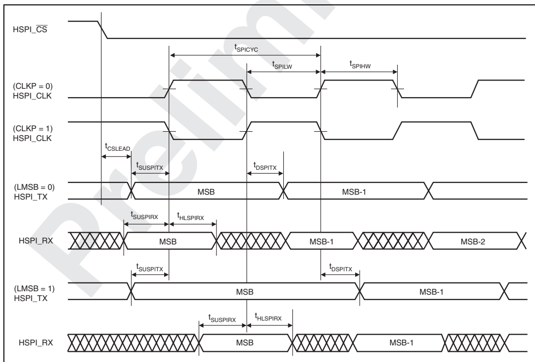
Figure 32.49 HSPI Data Output/Input Timing
