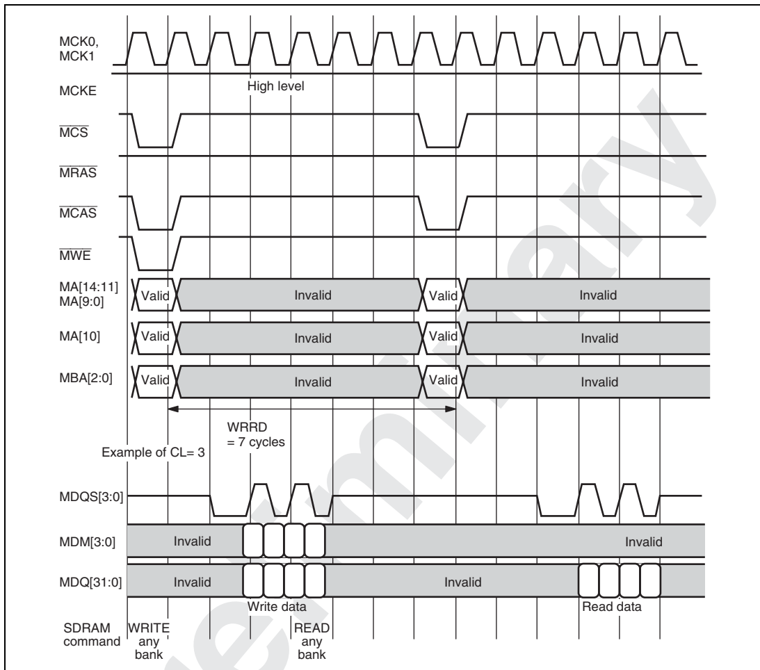
Figure 12.19 WRITE-READ Minimum Time
