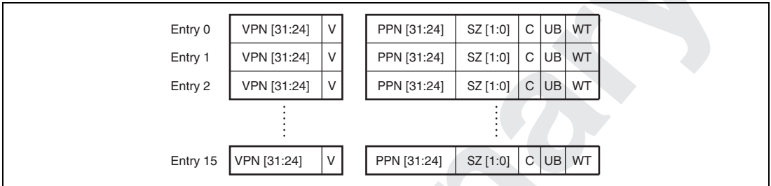
Figure 7.17 PMB Configuration
