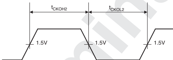
Figure 32.3 CLKOUT Clock Output Timing (2)
