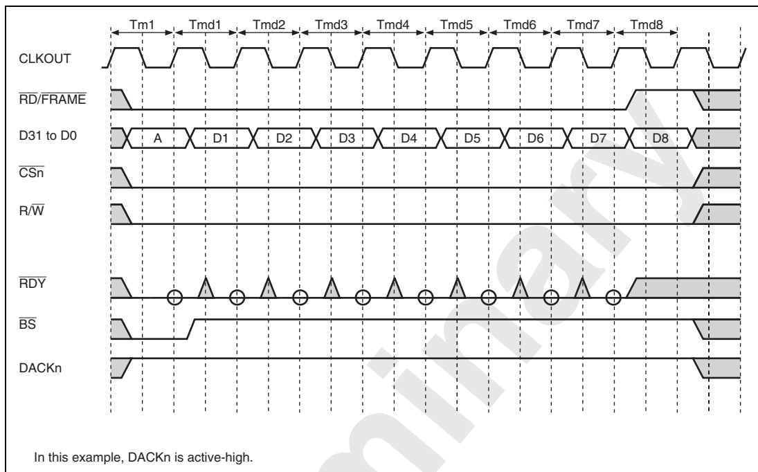
Figure 11.34 MPX Interface Timing 11 (Burst Write Cycle, IW = 0000, No External Wait, 32-Bit Bus Width, 32-Byte Data Transfer)
