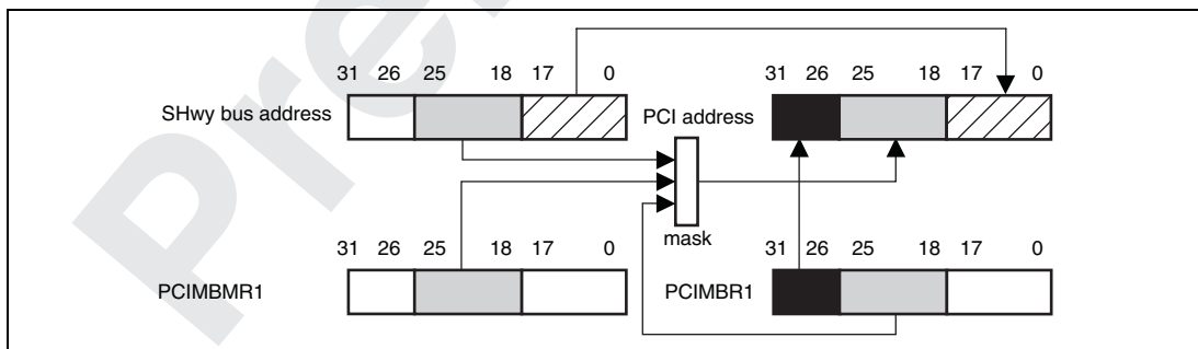
Figure 13.4 Access from SHwy Bus to PCI Memory (PCI Bus) (PCI Memory Space 1)
