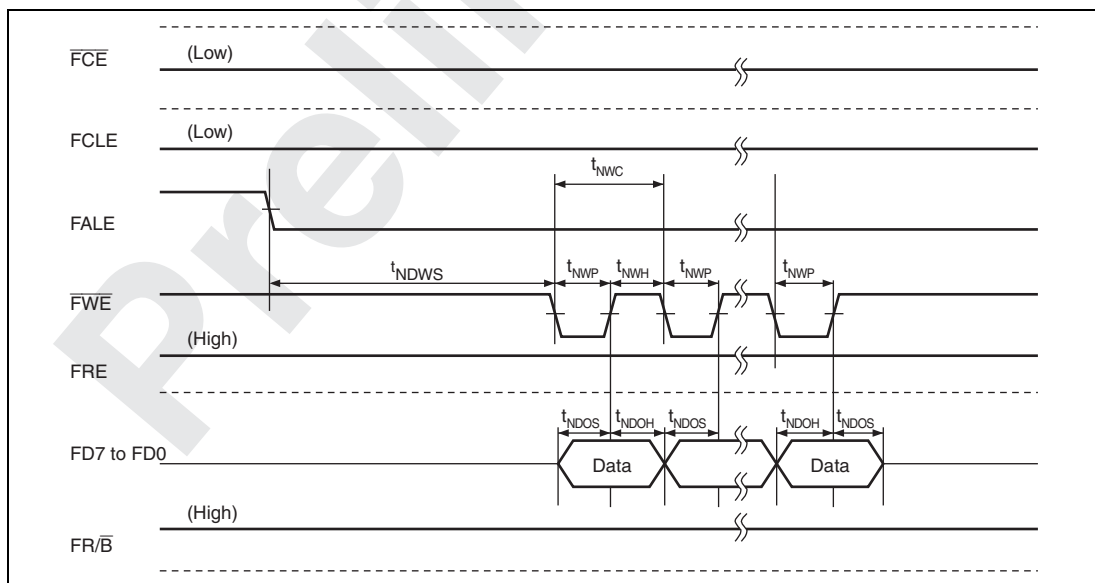
Figure 32.71 Data Write Timing of NAND-Type Flash Memory
