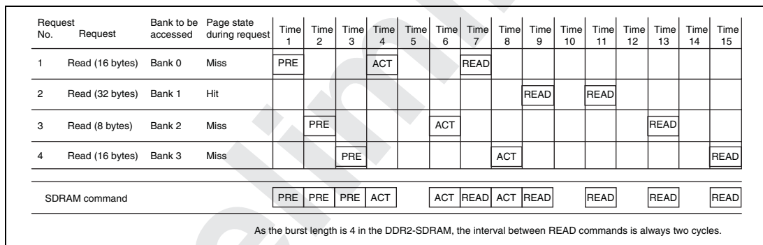
Figure 12.6 Example of Preceding Precharge/Activate Processing
