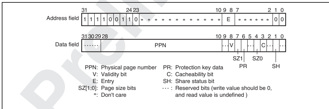
Figure 7.13 Memory-Mapped ITLB Data Array
