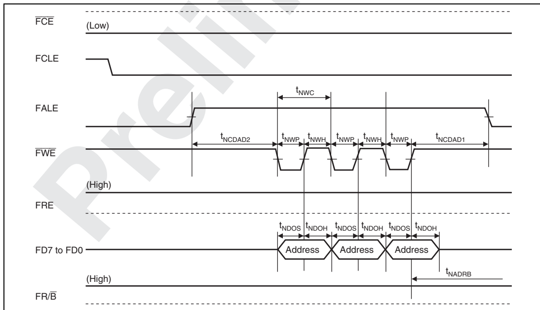
Figure 32.69 Address Issue Timing of NAND-Type Flash Memory
