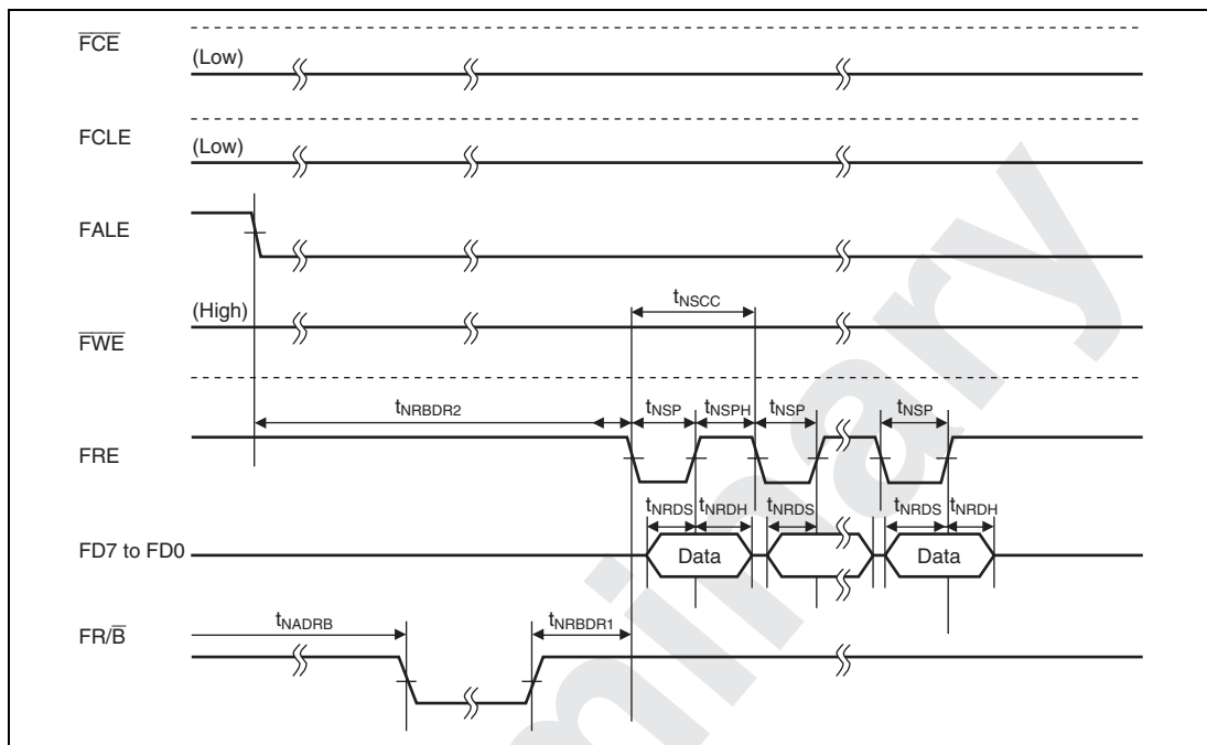
Figure 32.70 Data Read Timing of NAND-Type Flash Memory
