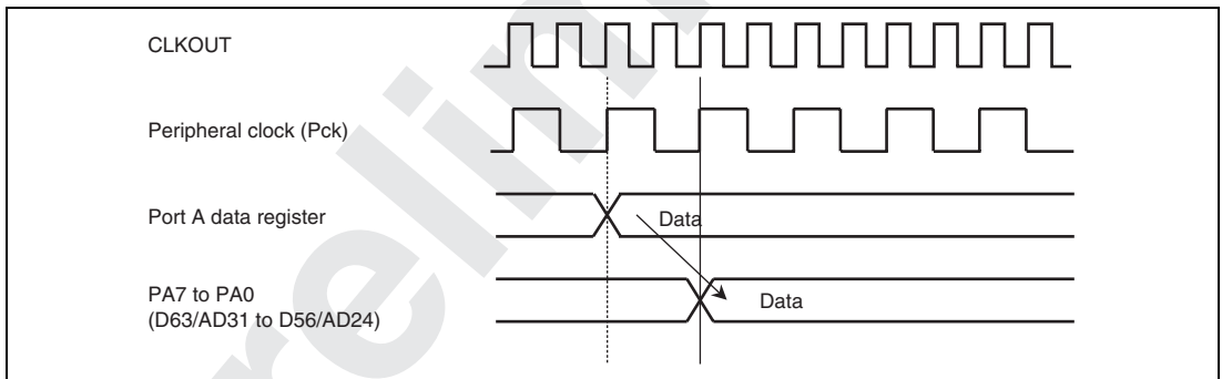
Figure 28.1 Port A Data Output Timing Diagram
