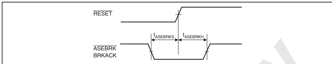
Figure 32.45 \overline{\text{RESET}} Hold Timing
