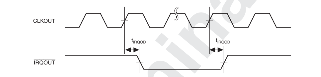
Figure 32.36 \overline{\text{IRQOUT}} Timing
