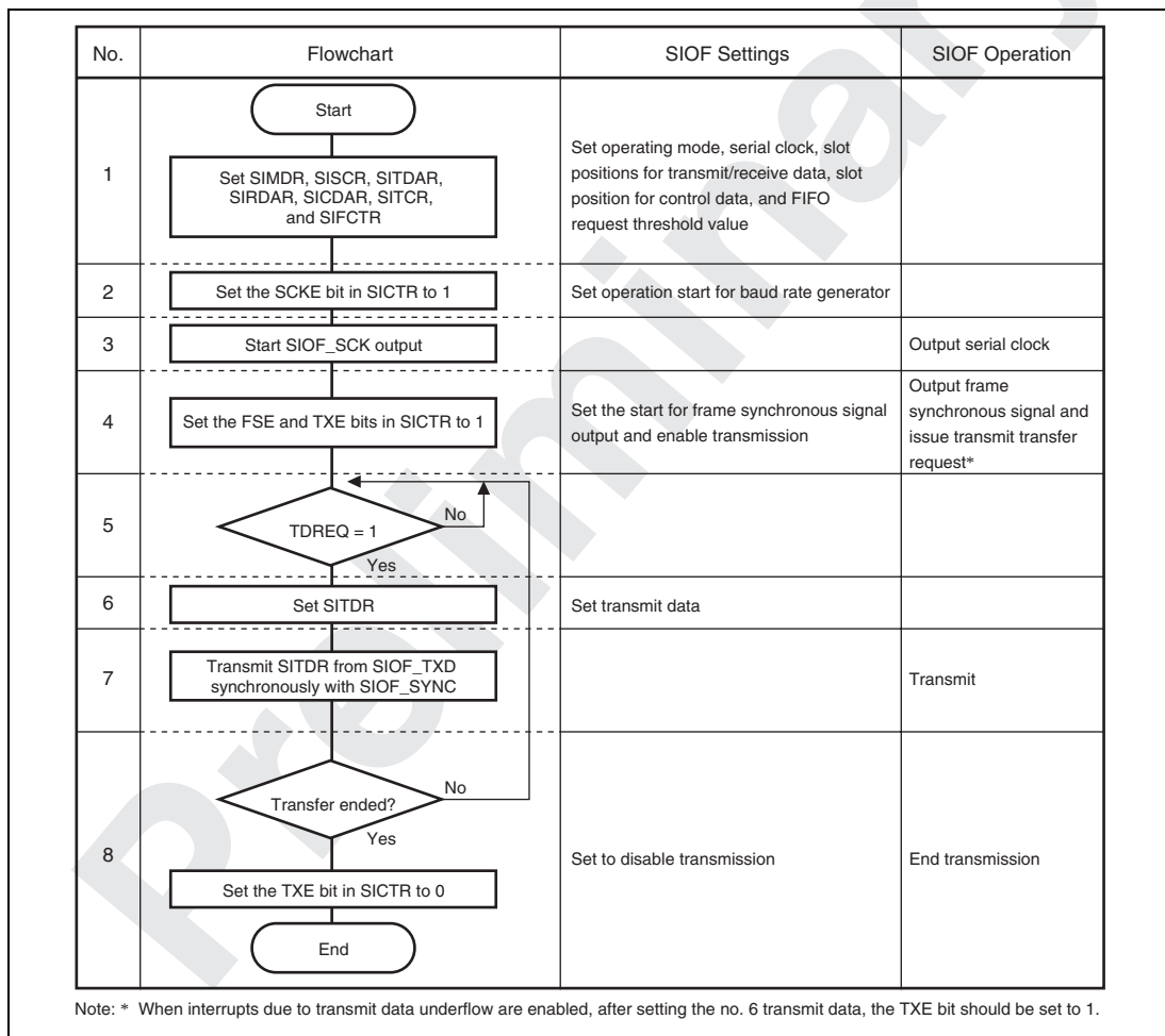
Figure 22.9 Example of Transmit Operation in Master Mode
