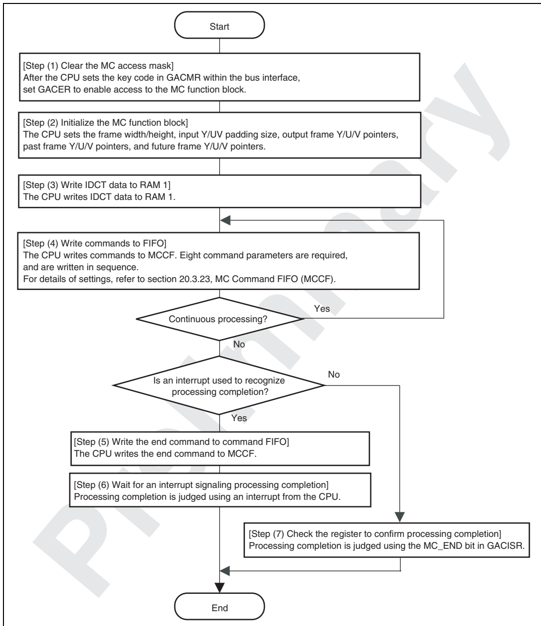
Figure 20.7 MC Processing Procedure
