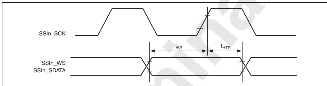
Figure 32.66 SSI Reception Timing (1)
