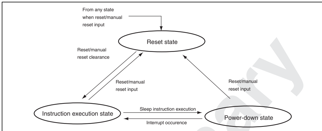
Figure 2.8 Processing State Transitions
