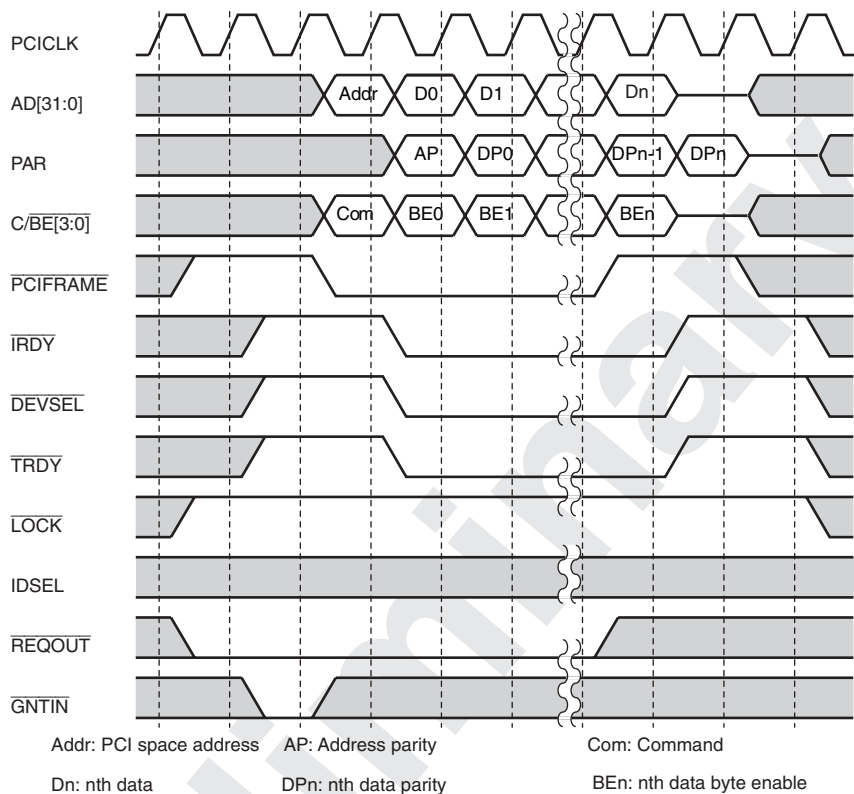
Figure 13.21 Master Write Cycle in Normal Mode (Burst)
