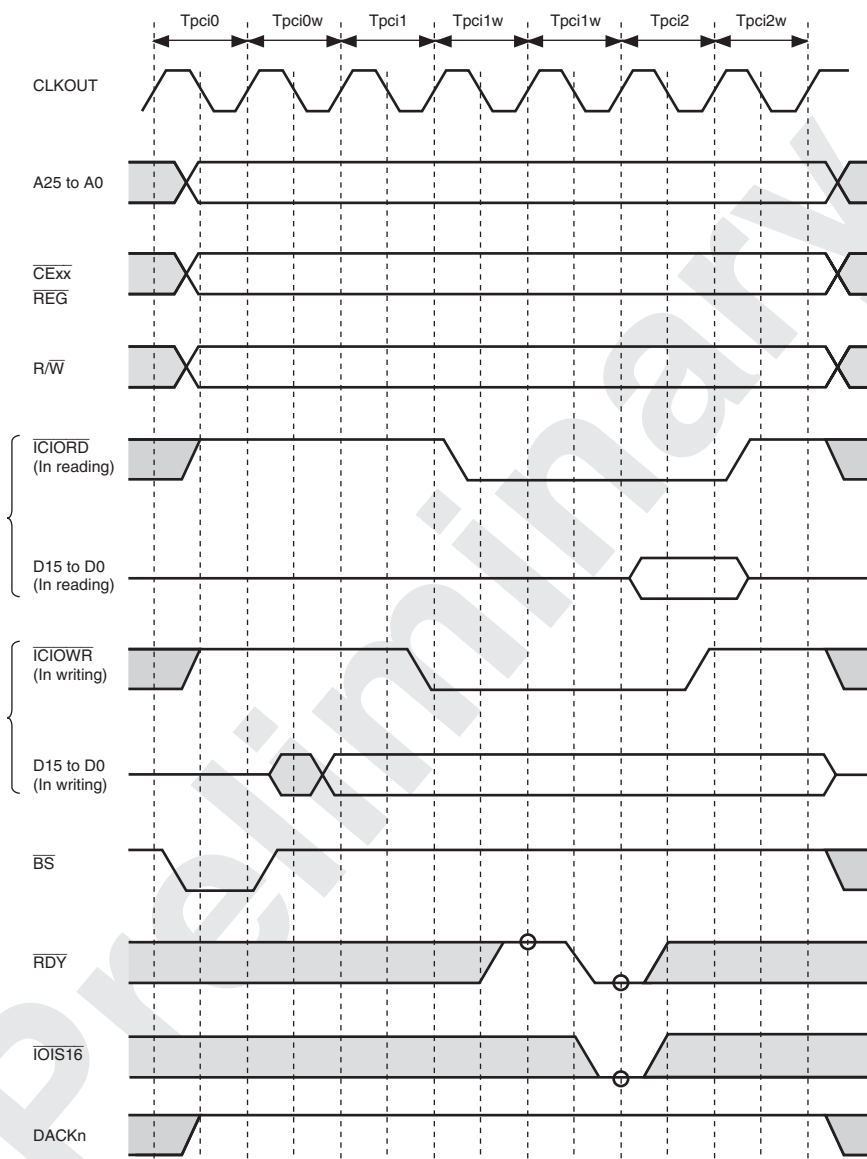
Figure 11.20 Wait Timing for PCMCIA I/O Card Interface
