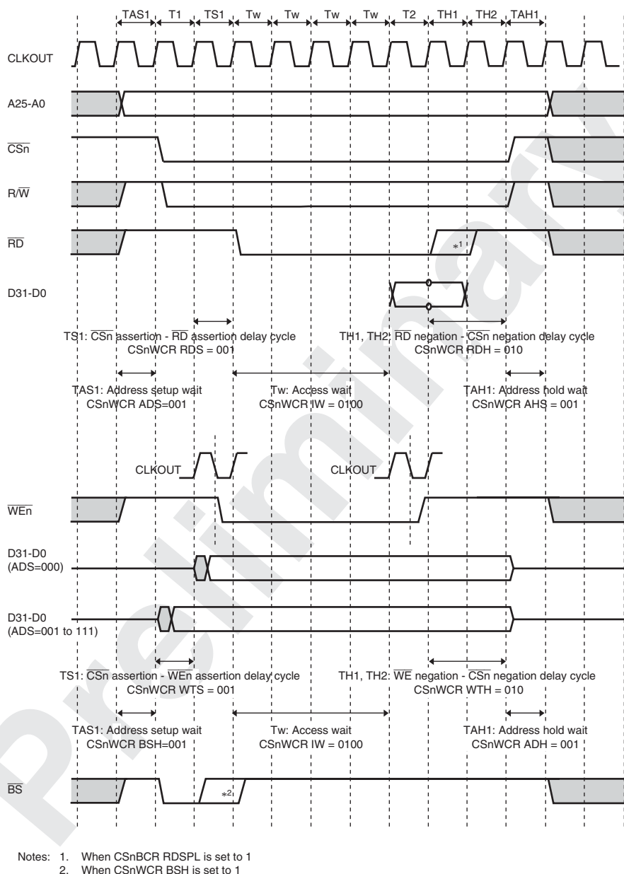
Figure 11.11 SRAM Interface Wait Timing (Read-Strobe Negate Timing Setting)
