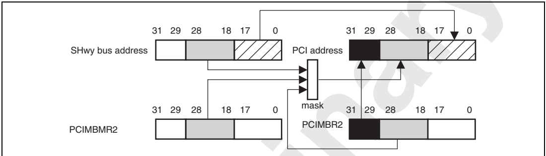
Figure 13.5 Access from SHwy Bus to PCI Memory (PCI Bus) (PCI Memory Space 2)
