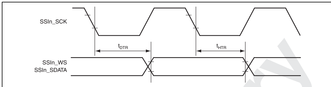
Figure 32.65 SSI Transmission Timing (2)
