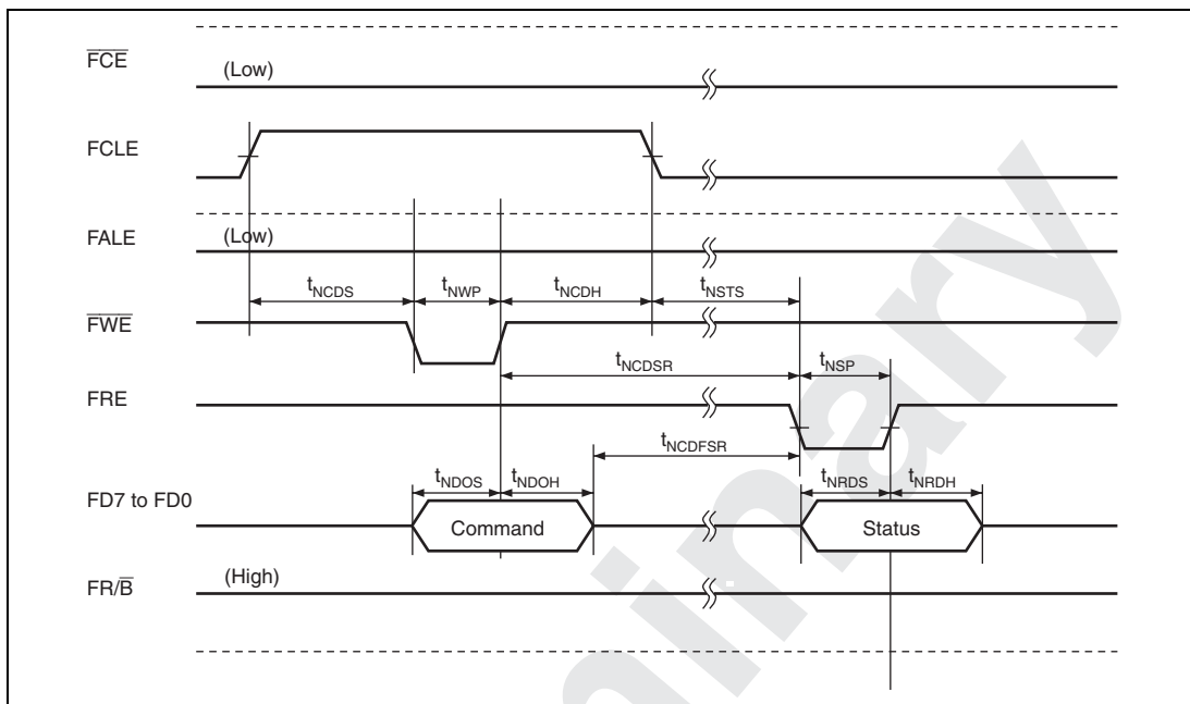
Figure 32.72 Status Read Timing of NAND-Type Flash Memory
