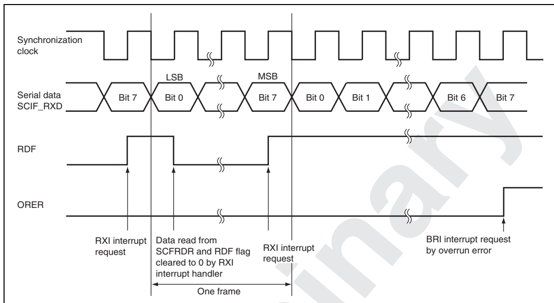
Figure 21.20 Example of SCIF Reception Operation
