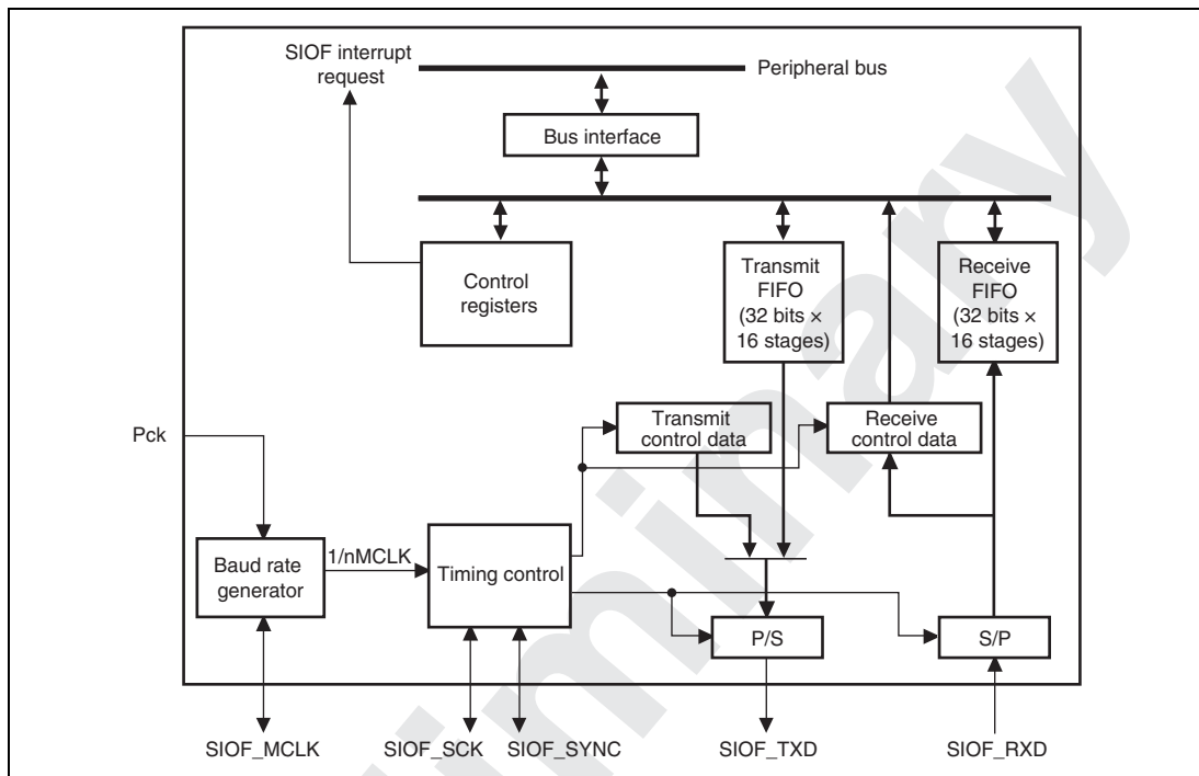
Figure 22.1 Block Diagram of SIOF
