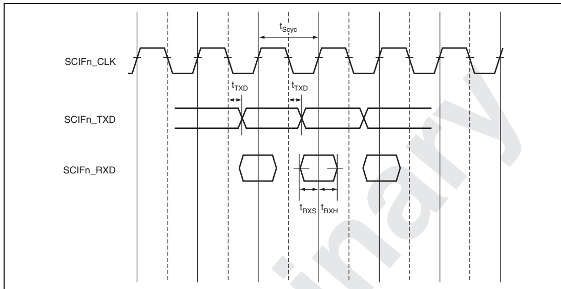
Figure 32.43 Clock Timing in SCIF I/O Synchronous Mode
