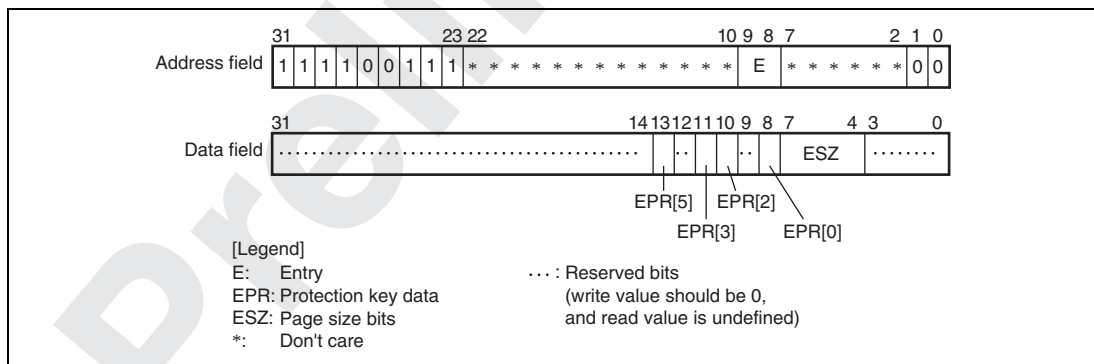
Figure D.10 Memory-Mapped ITLB Data Array 2 (TLB Extended Mode)
