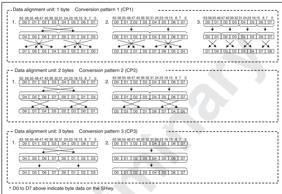
Figure 20.8 Data Alignment Conversion Pattern
