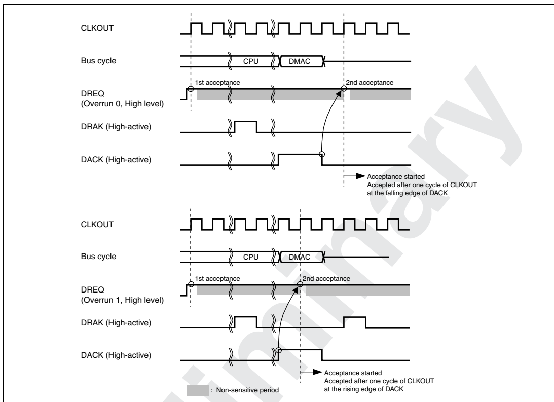
Figure 14.20 Example 1 of DREQ Input Detection in Burst Mode Level Detection (Byte Transfer in 8/16/32/64-Bit Bus Width, Word Transfer in 16/32/64-Bit Bus Width, or Longword Transfer in 32/64-Bit Bus Width)
