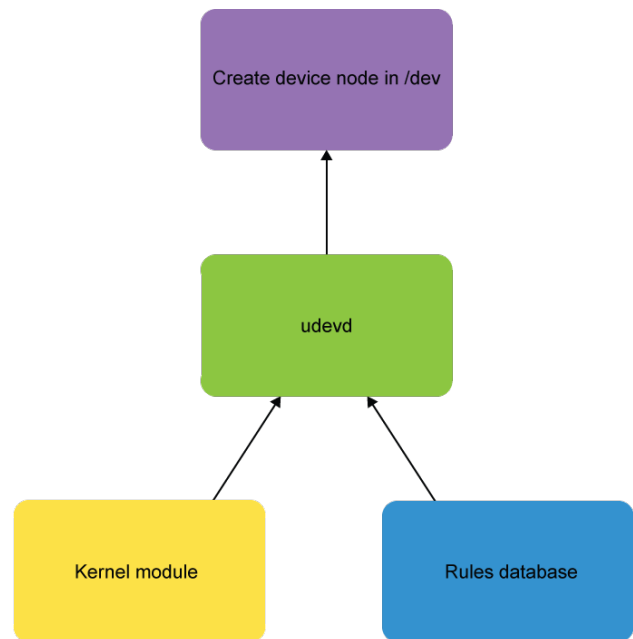
Figure 26.2: udev Rules
