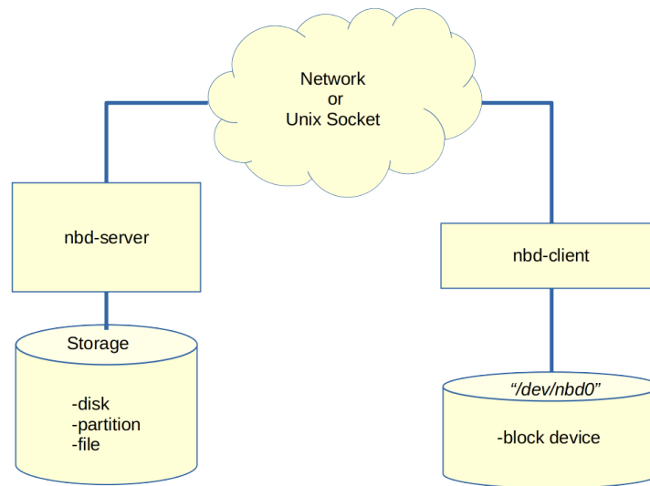
Figure 21.9: Network Block Device
