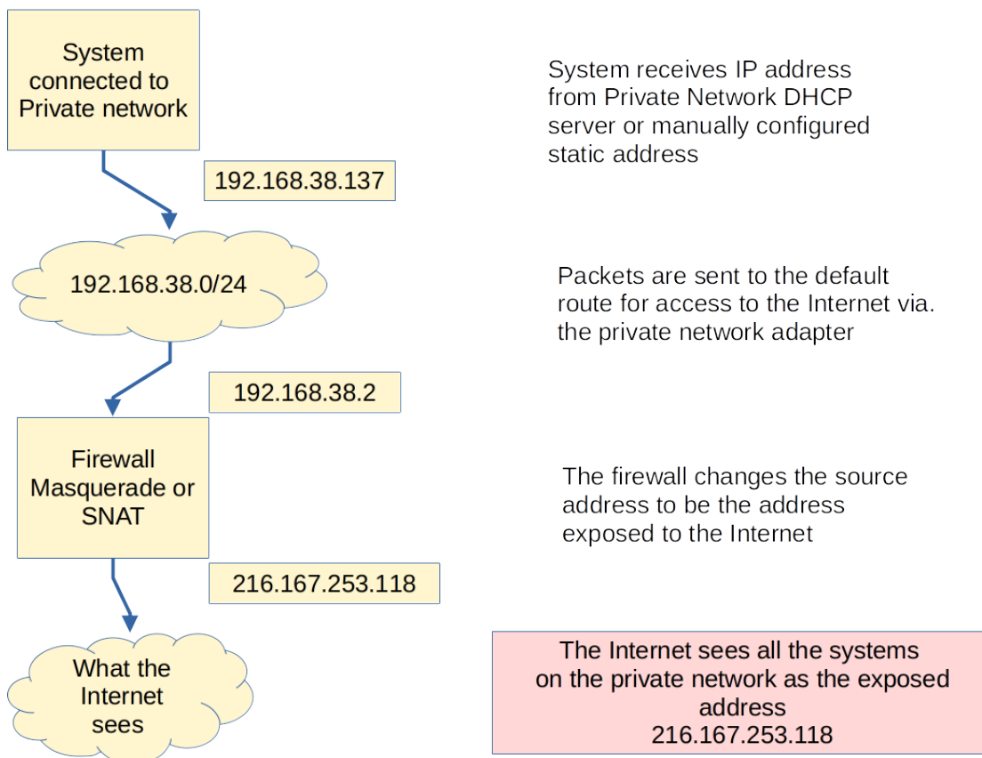
Figure 30.3: SNAT or MASQUERADE example
