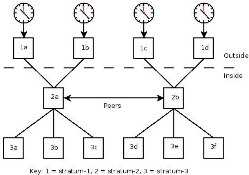
Figure 27.2: Network Time Protocol
