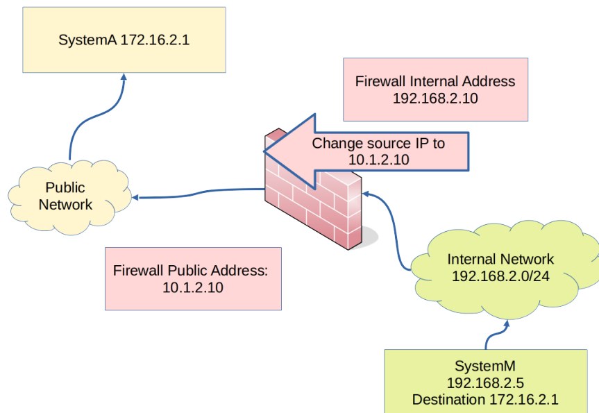
Figure 30.2: Source NAT and MASQUERADE
