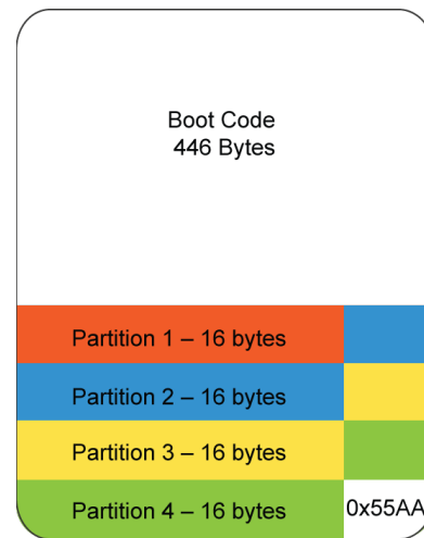
Figure 20.2: MBR Disk Partition Table
