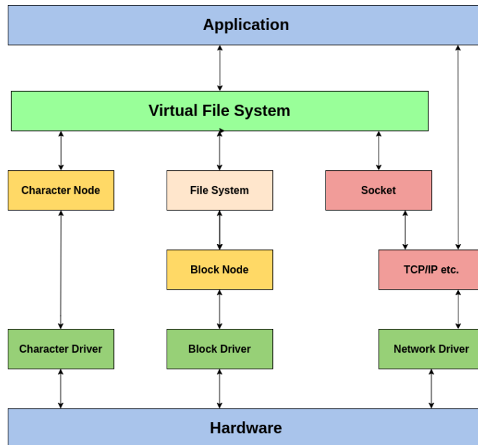
Figure 26.1: Device Nodes
