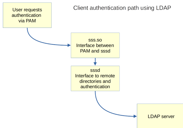
Figure 29.1: LDAP Client Authentication Process
