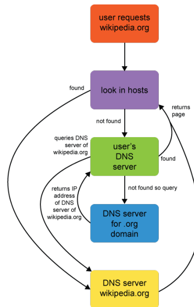
Figure 28.5: DNS
