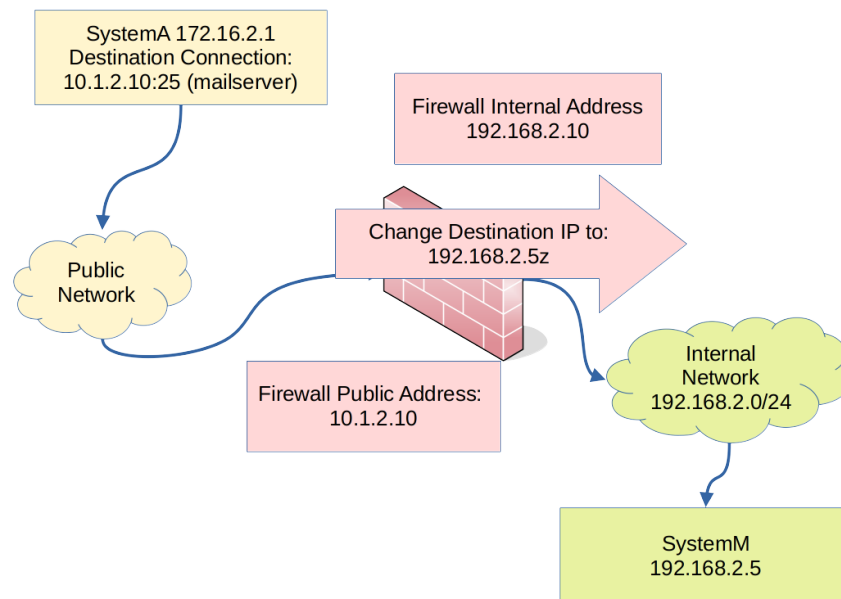
Figure 30.1: Destination NAT
