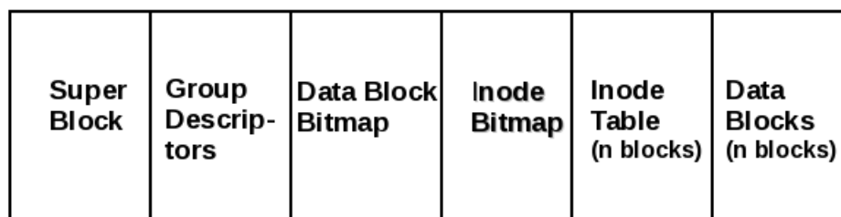
Figure 22.1: ext[3,4] Filesystem Layout
