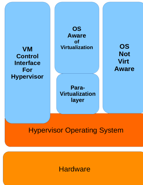
Figure 19.2: Dedicated Hypervisor
