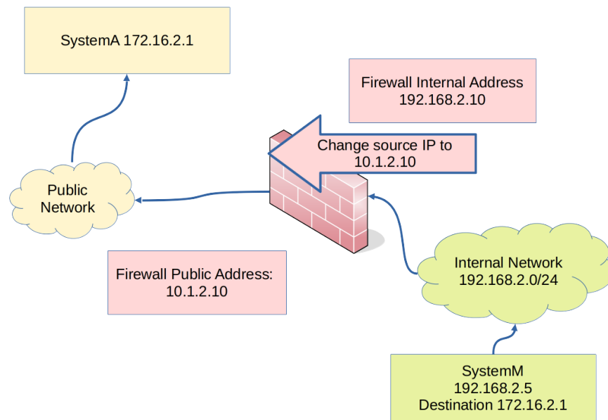
Figure 32.2: Source NAT and Masquerade
