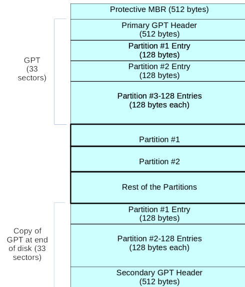
Figure 22.3: GPT Disk Partition Table
