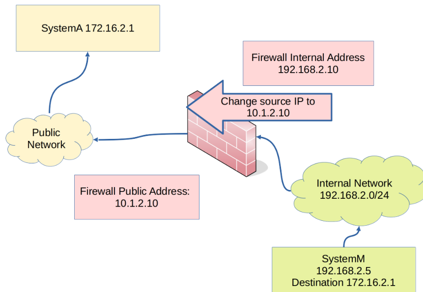
Figure 32.2: Source NAT and Masquerade
