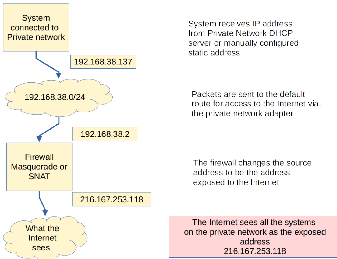
Figure 32.3: SNAT or MASQUERADE example
