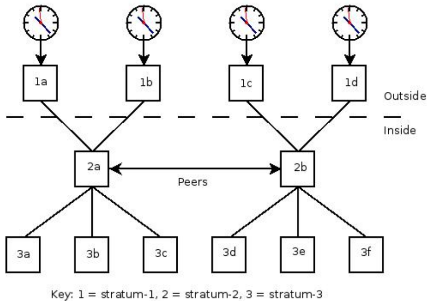
Figure 29.2: Network Time Protocol
