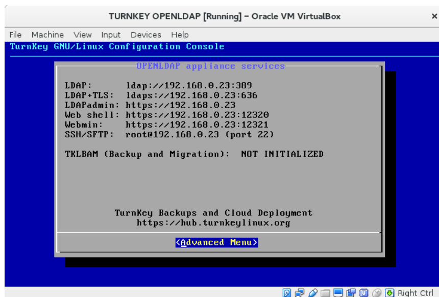
Figure 31.2: Turnkey OpenLDAP Appliance Services
