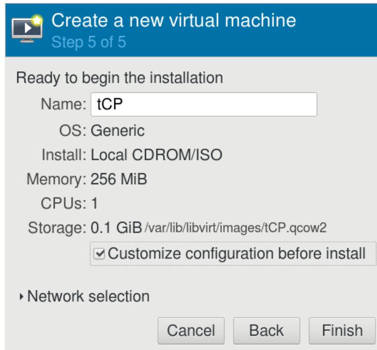
Figure 19.10: Beginning the VM installation in virt-manager
