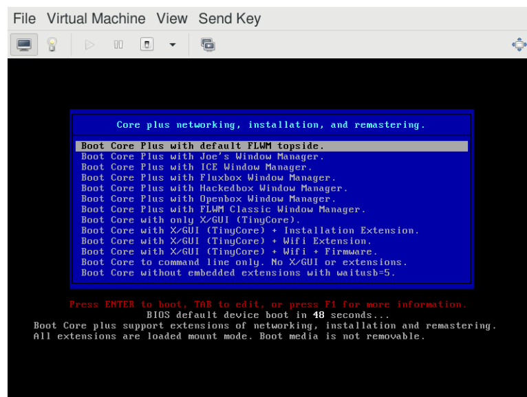
Figure 19.12: Booting into the Installation Media with virt-manager
