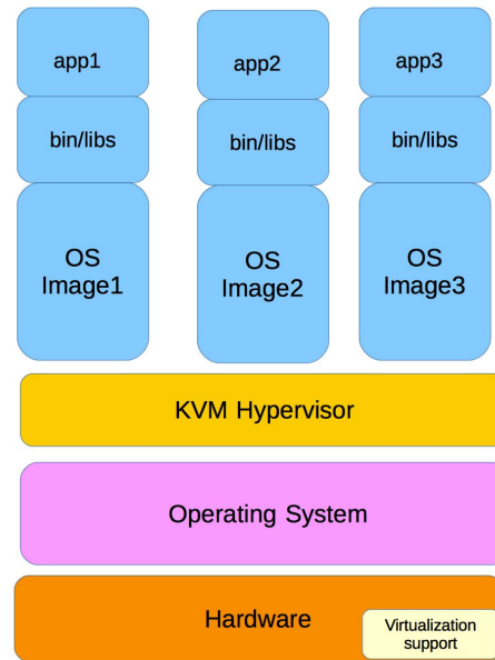
Figure 19.3: Hypervisor in the Kernel
