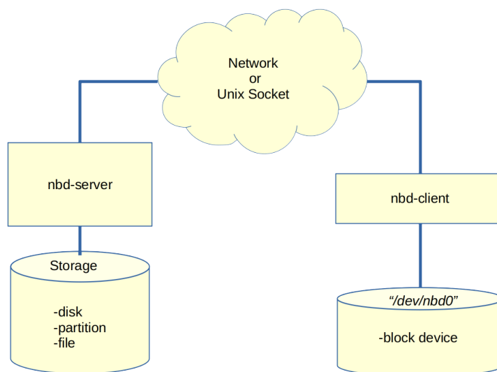
Figure 23.9: Network Block Device
