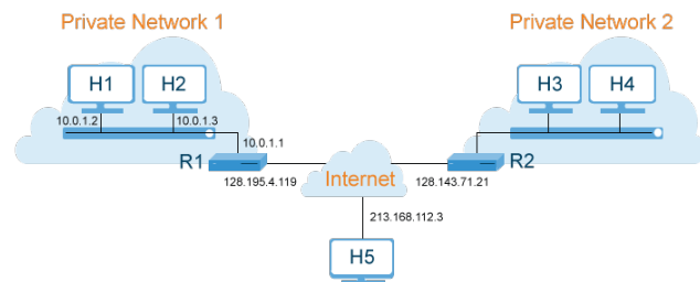
Figure 29.1: IP Addresses
