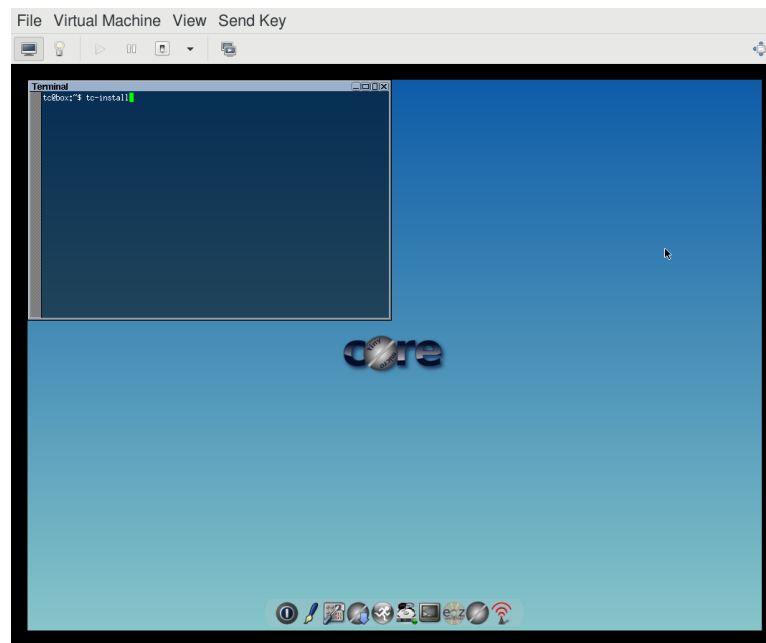
Figure 19.15: Running tc-install
