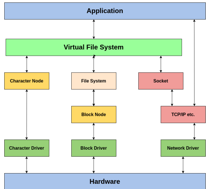
Figure 2.3: Device Nodes
