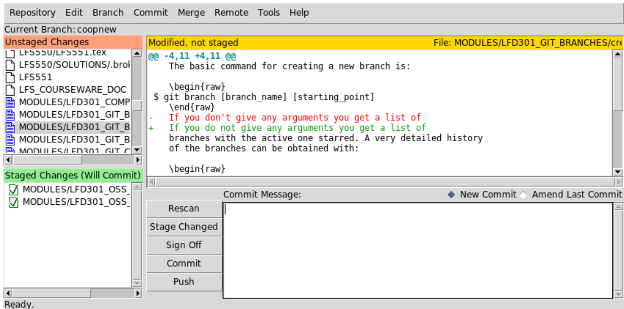
Figure 13.1: git gui
