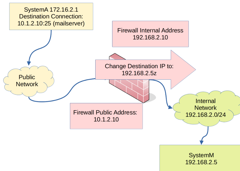
Figure 32.1: Destination NAT
