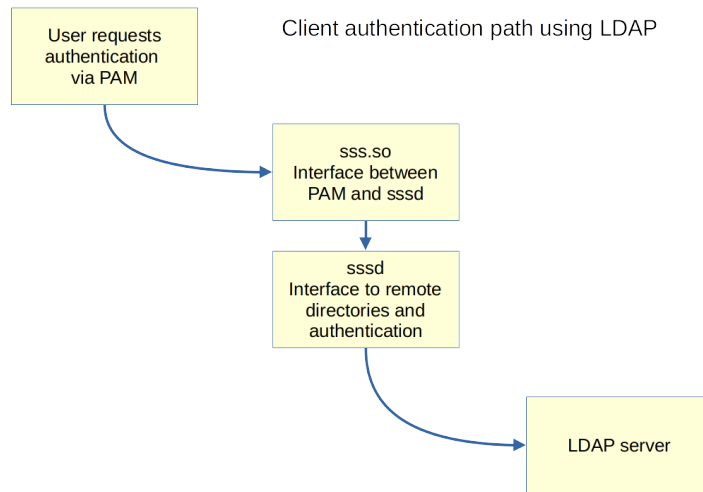
Figure 31.1: LDAP Client Authentication Process
