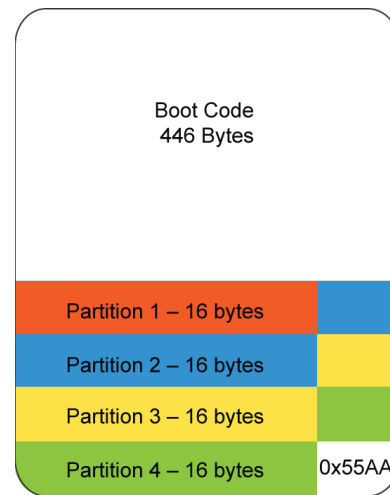
Figure 22.2: MBR Disk Partition Table
