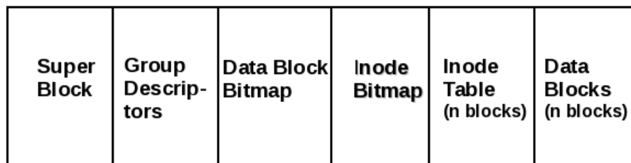
Figure 24.1: ext[3,4] Filesystem Layout
