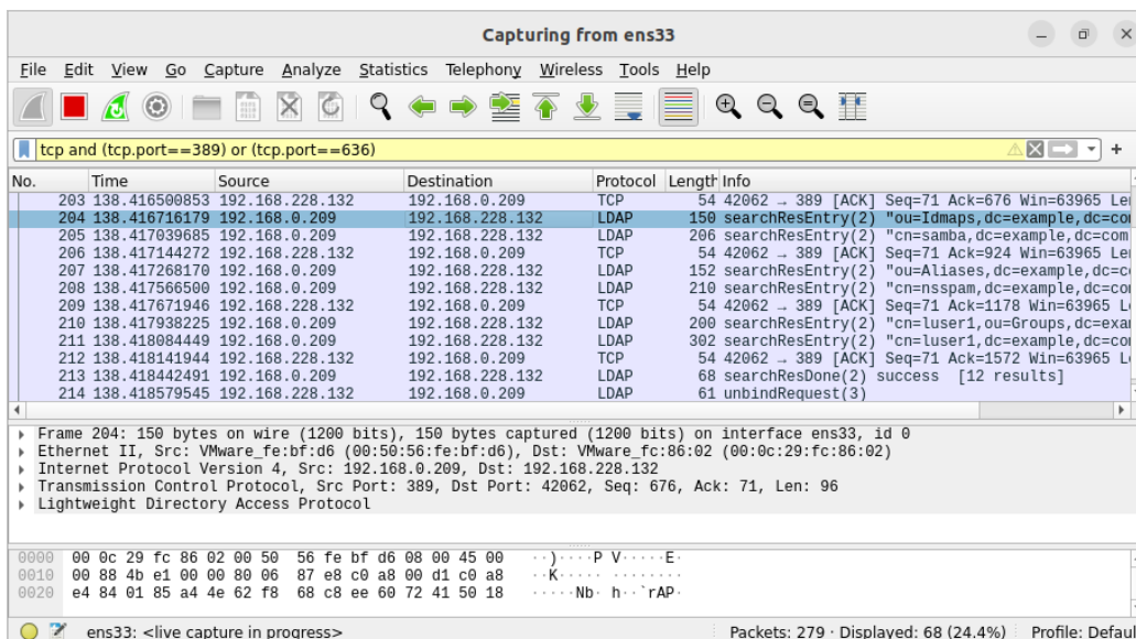
Figure 31.3: Wireshark LDAP packet trace
