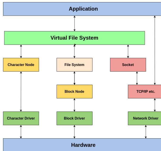
Figure 28.1: Device Nodes
