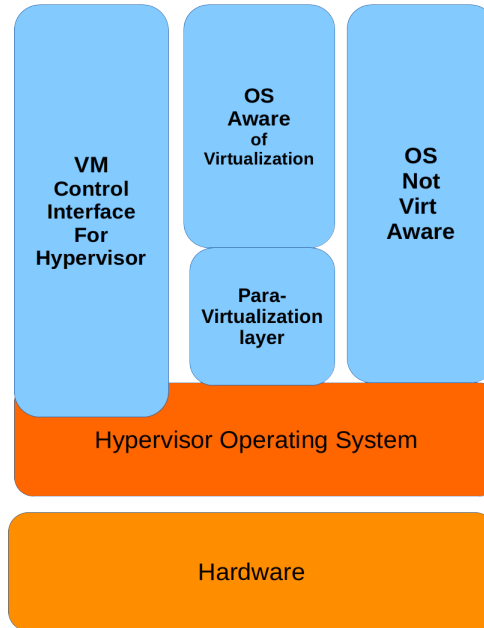
Figure 19.2: Dedicated Hypervisor
