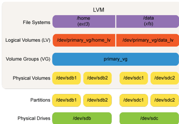
Figure 25.1: LVM components
