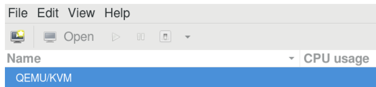
Figure 19.5: Starting virt-manager
