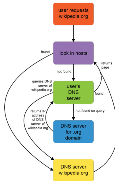
Figure 30.8: DNS
