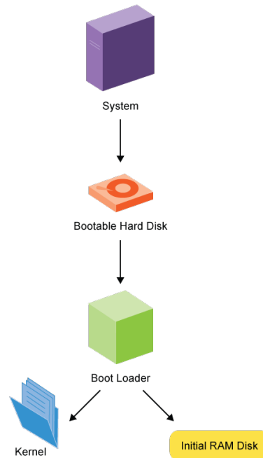
図 37.1: Boot Sequence
