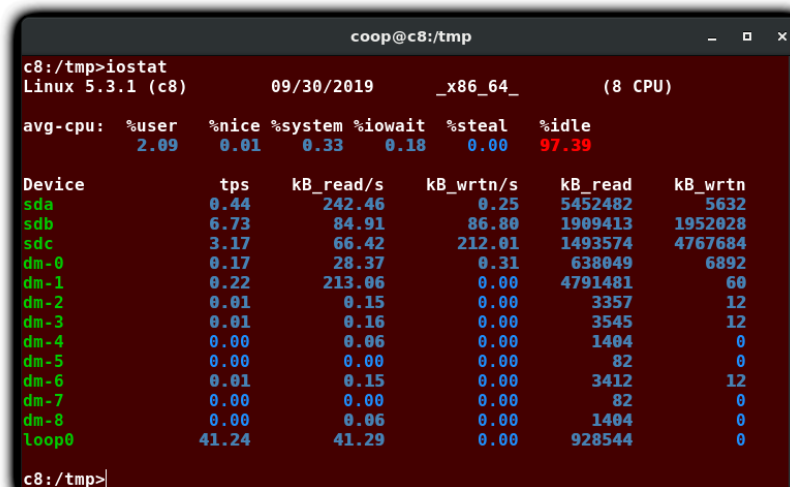
Figure 14.1: iostat
